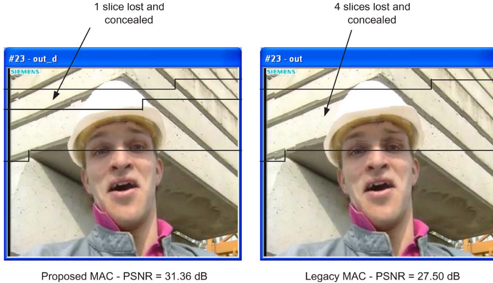
Fig. 5. Four NAL units per MAC frame at PER = 9.5 \cdot 10^{-3} , with concealment.
