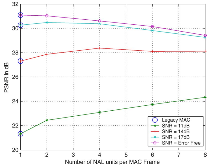
Fig. 8. PSNR comparison versus the number of NAL units for the proposed MAC with no ARQ ( foreman at 128 kb/s).
