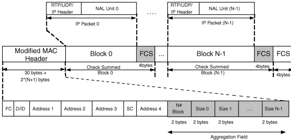
Fig. 3. MAC frame modification for multiple NAL unit MAC packetization.
