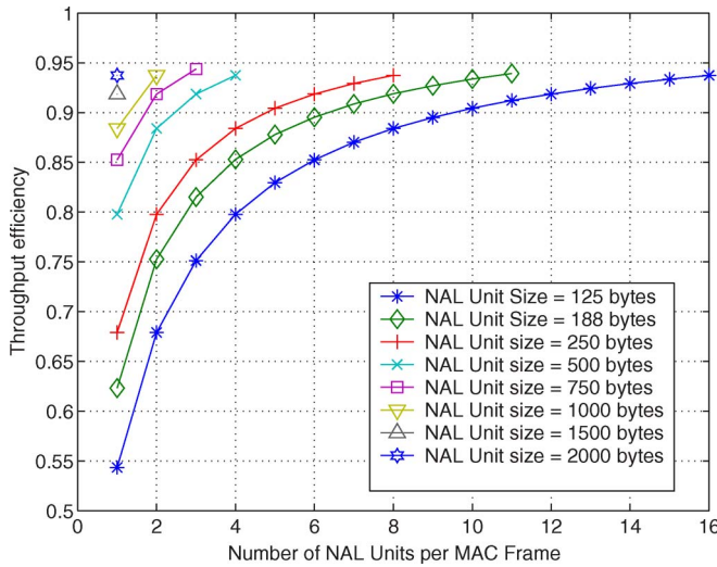
Fig. 1. Throughput efficiency. BPSK 1/2 rate. Different numbers of NAL units per MAC frame.
