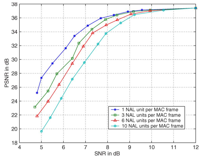
Fig. 2. PSNR with the IEEE 802.11 legacy MAC with one ARQ allowed.
