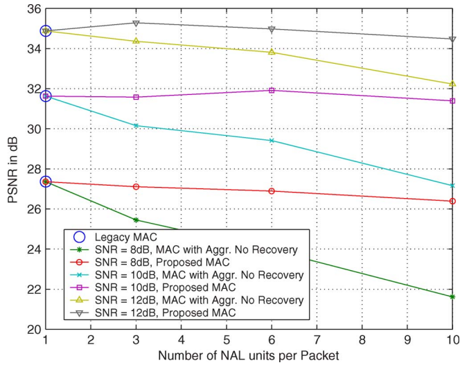
Fig. 6. PSNR comparison of the IEEE 802.11 legacy MAC/proposed MAC without ARQ for different SNR values (fixed NAL size).
