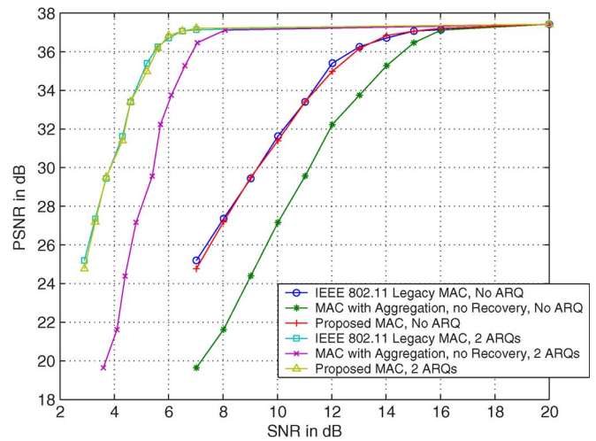
Fig. 4. PSNR comparison of the IEEE 802.11 legacy MAC/proposed MAC.
