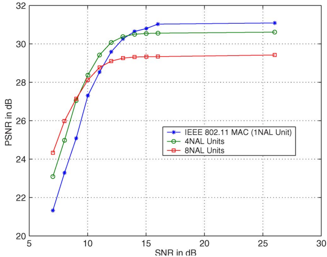
Fig. 7. PSNR comparison versus the SNR for the proposed MAC with no ARQ ( foreman at 128 kb/s).
