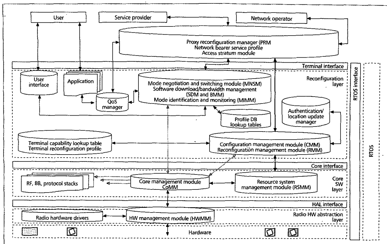
■ Figure 4. Terminal reconfiguration management architecture.
