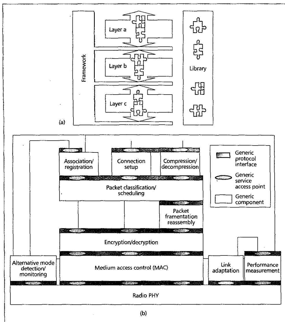
■ Figure 2. a) Composable protocol stack framework; b) an example of generic stack implementation.
