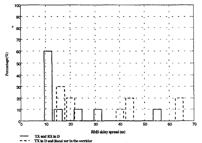
Figure 11 - Probability Distribution of RMS delay for different room transmission situation (Location G - omni:omni configuration).
