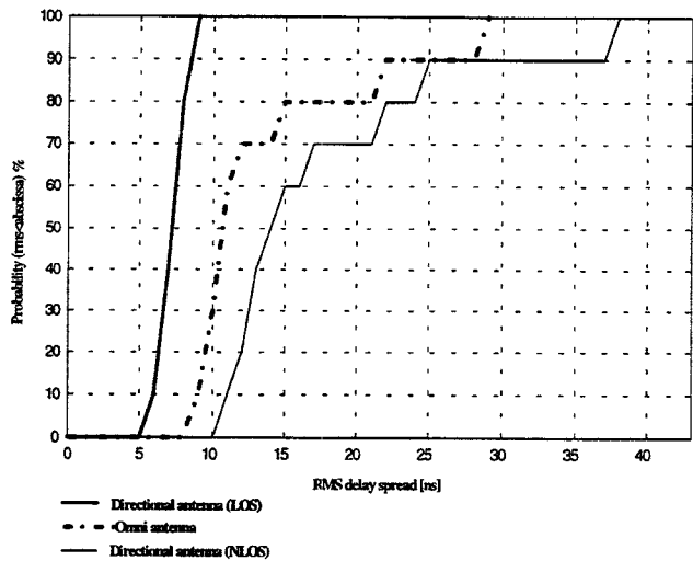
Figure 7 - Cumulative distributions for location D
