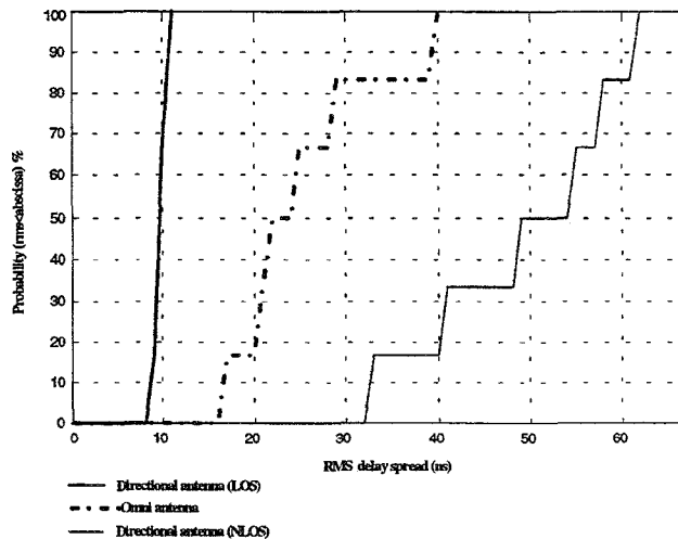
Figure 4 - Cumulative distributions for location A
