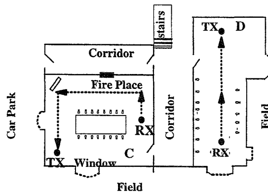
Figure 2 Plan of the measurement locations C and D
