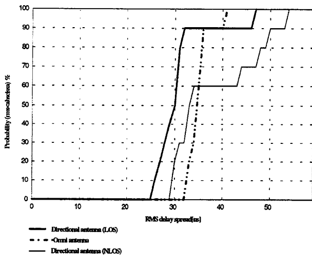
Figure 5 - Cumulative distributions for location B
