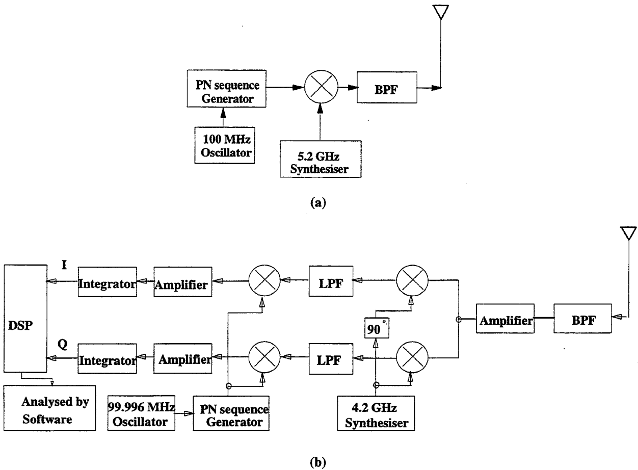
Figure 1 - Block diagram of the channel sounder (a) Transmitter (b) Receiver
