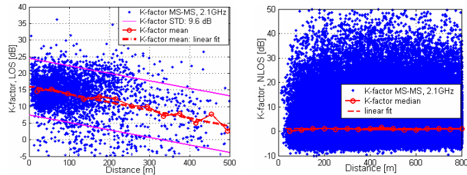
Figure 11. K-factor versus distance. LOS and NLOS
