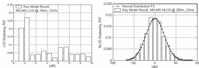
Figure 7. Shadowing PDF of LOS and NLOS, MS-MS at 2.1GHz
