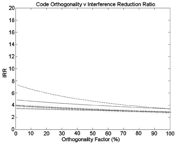
Fig. 11. IRR versus code orthogonality for a user located close to BS and cell boundary (an eight-beam antenna system is employed). System parameters are given in Tables I and II. - \cdot - \cdot - is intracell user signal orthogonality, + + + + is intercell user signal orthogonality, - is intracell pilot signal orthogonality, and \cdot \cdot \cdot \cdot \cdot is intercell pilot-signal orthogonality.
