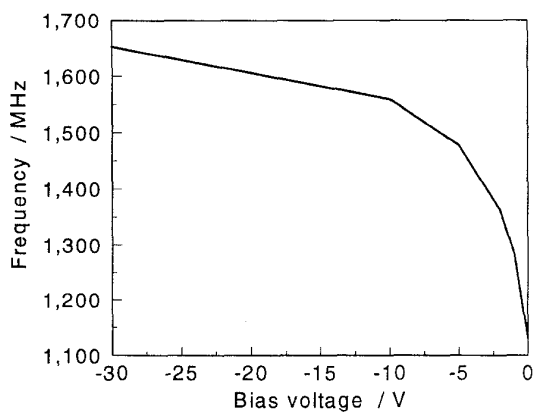
Fig.2 Resonant frequency versus applied bias voltage.
