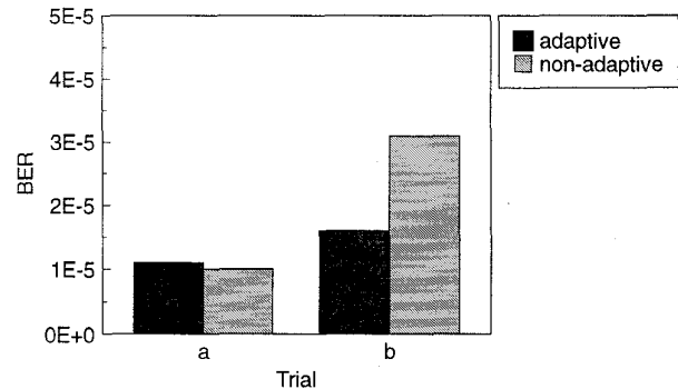
Fig.9 Bit error rate measurements of adaptive and non-adaptive antennas (no Doppler shift) a) undisturbed b) disturbed.
