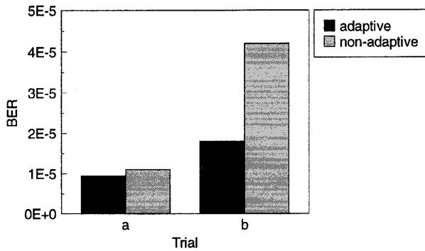
Fig.11 Bit error rate measurements of adaptive and non-adaptive antennas (including Doppler shift) a) undisturbed b) disturbed.
