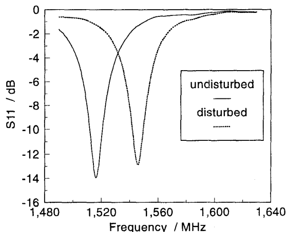
Fig.5 Reflected power versus frequency for undisturbed and disturbed antenna.
