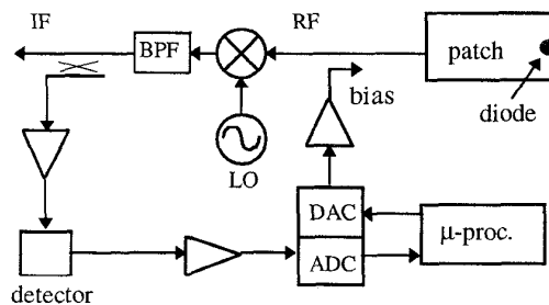
Fig.4 Block diagram of receiving adaptive frequency tunable antenna.
