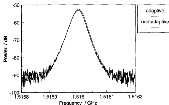
Fig.6 Transmitted power of undisturbed adaptive and non-adaptive antenna.
