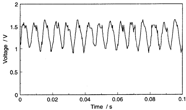
Fig.10 Input to ADC when Doppler shift applied.
