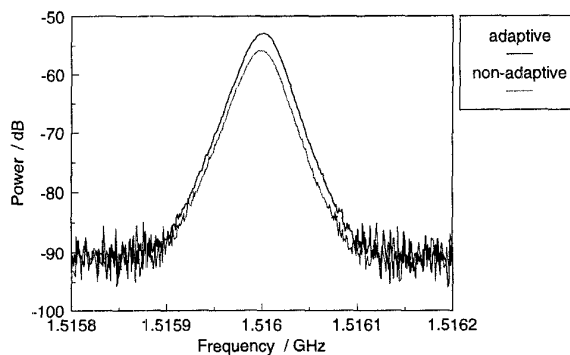
Fig.7 Transmitted power of disturbed adaptive and non-adaptive antenna.
