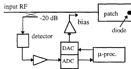
Fig.3 Block diagram of transmitting adaptive frequency tunable antenna.
