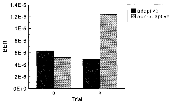
Fig.8 Measured BER of adaptive and non-adaptive antenna a) undisturbed, b) disturbed.
