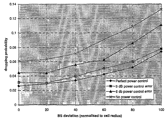
Figure 3: Network performance with power control error
