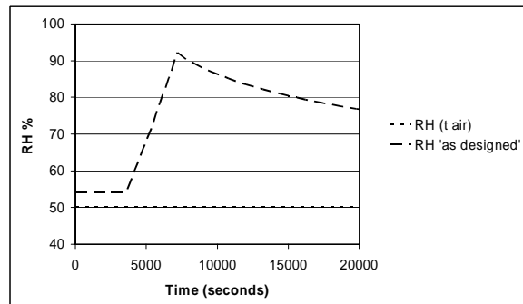
Figure 4. Predicted surface RH for the ‘standard’ RCD.
