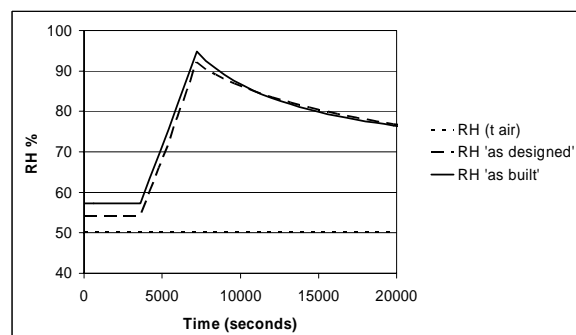
Figure 8. Comparison of predicted surface RH
