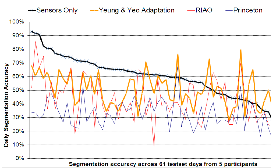
Figure 4. Performance in identifying boundaries between lifelog events. The x-axis sorted in descending order of performance of our “Sensors Only” approach represents 61 discrete days from 5 individuals, and the y-axis represents the event-segmentation F1-measure accuracy obtained for each of those 61 days. Our method in the thick black line represents an improvement over existing techniques
