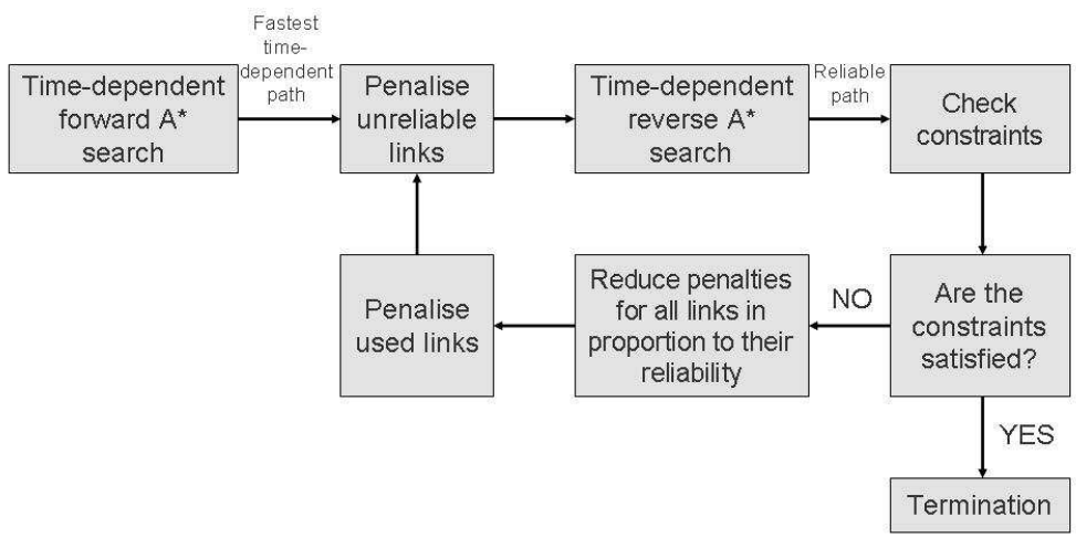
The modified link penalty method
