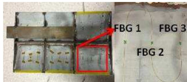
Fig. 8. Inner surface of a rudder mapped with 12 FBGs for acoustic emission monitoring.
