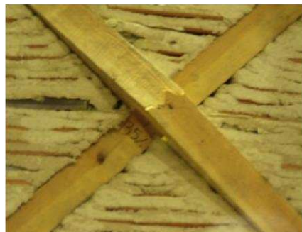
Figure 25 Buckling and cracking of diagonal.
