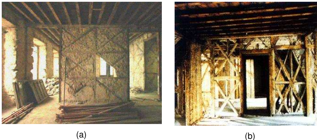
Figure 1 A “Pombalino” building: a) Interior view of; b) “Frontal” panel inside the building.
