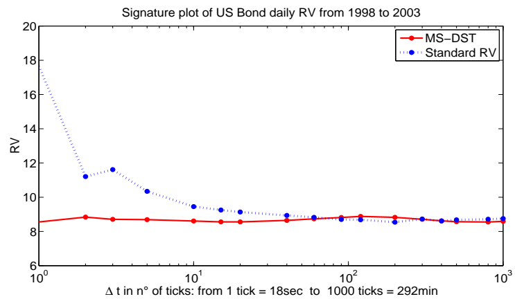
Figure 7: Signature Plot in semilog scale of the standard (dotted) and DST (solid) realized volatility for S&P 500, FIB 30 and US Bond from January 1998 to October 2003.
