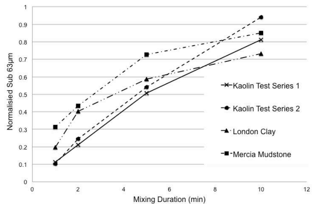
Figure 5 Percentage of sub 63 μm particles pass at increasing mixing times normalised against fully dispersed data.
