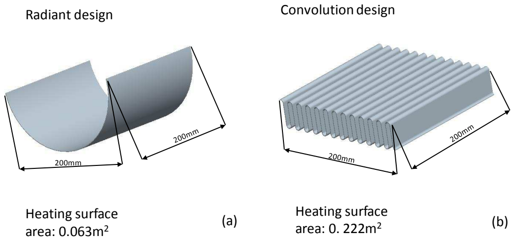
Fig 5 Radiant design and convoluted design for HHX with same projection area of 200 mm by 200 mm. (a) Radiant design heating surface area is 0.063 m 2 ; (b) Convoluted design heating surface area is 0.222 m 2
