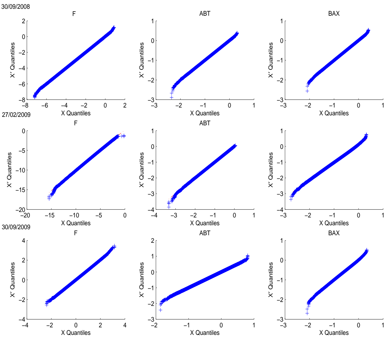
Figure 1 Convolution error: recovering the VG distribution.
