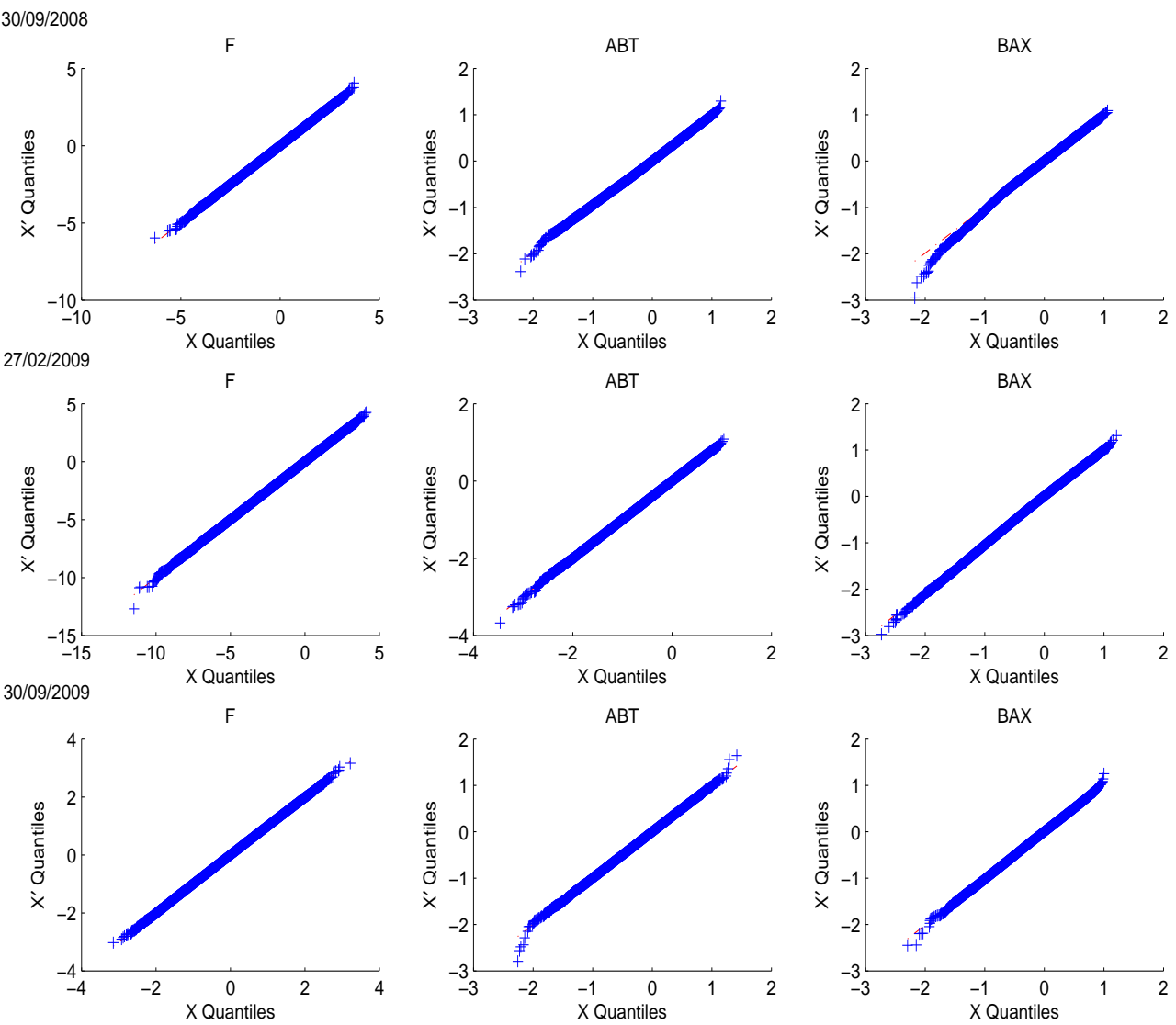
Figure 2 Convolution error: recovering the VG distribution.
