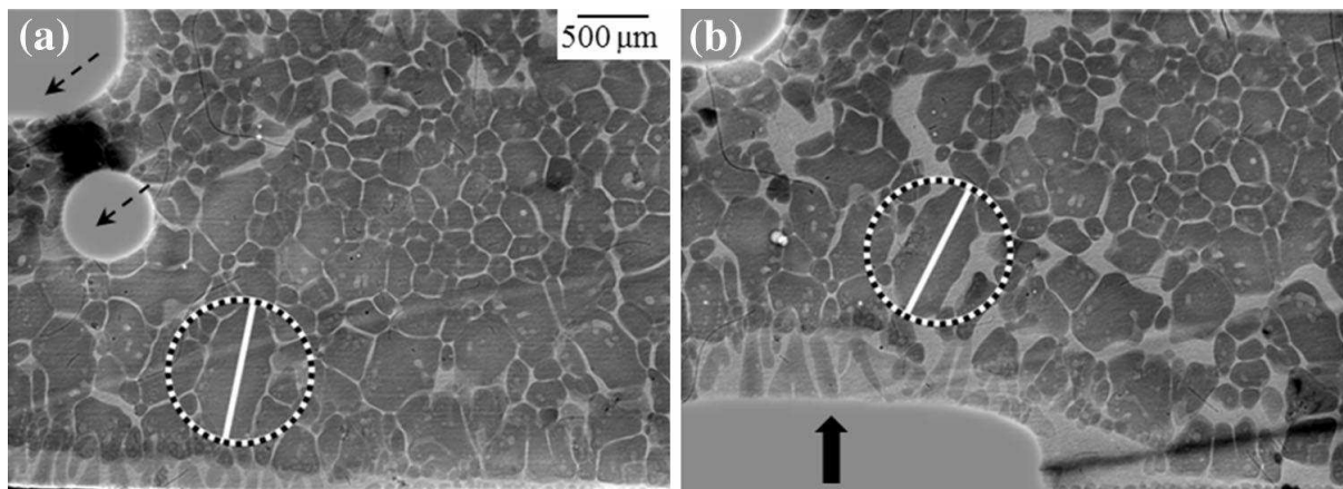
Figure 5. Deformation of globular–polygonal Fe-2C-1Mn-0.5Si at \sim 88\% solid: (a) prior to deformation and (b) after 1072 \mu\text{m} (3.1 mean grains) of push-plate displacement. Note the significantly enlarged liquid-filled interstices in (b) due to shear-induced dilation. The primary axis and circle of rotation are shown for a large grain with high aspect ratio. Austenite is dark gray, liquid is light gray, and the rounded features marked with arrows are pores.
