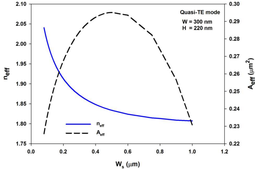
Fig. 4. Variations of the effective index, n_{\text{eff}} , and effective area, A_{\text{eff}} , with the slot width, W_s .
