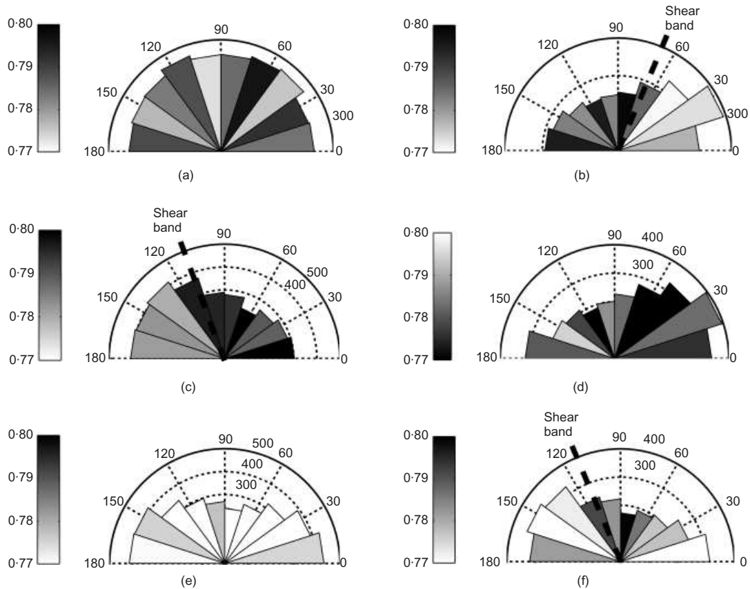
Fig. 4. Rose diagrams giving evolution of particle orientations during loading (shading indicates average aspect ratios of particles oriented within each angular bin): (a) vertical ( x-z ) plane Int-3-a; (b) vertical ( x-z ) plane Int-3-b-S; (c) vertical ( x-z ) plane Int-4-b-S; (d) vertical ( y-z ) plane Rec-3-a; (e) vertical ( x-z ) plane Rec-3-b; (f) vertical ( x-z ) plane Rec-4-S
