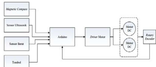
Gambar 8. Diagram Blok Hardware Sistem
