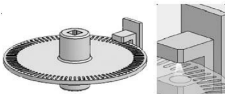
Gambar 5. Rotary Encoder[8]
