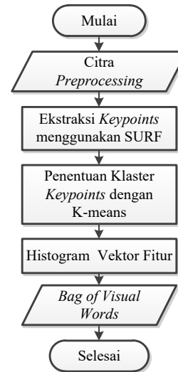
Gambar 7. Alur tahap Bag of Visual Words
