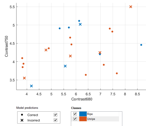
Gambar 3. Scatter plot data latih
