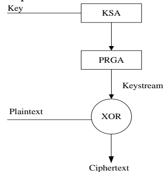
Gambar 1. Blok Diagram Algoritma RC4
