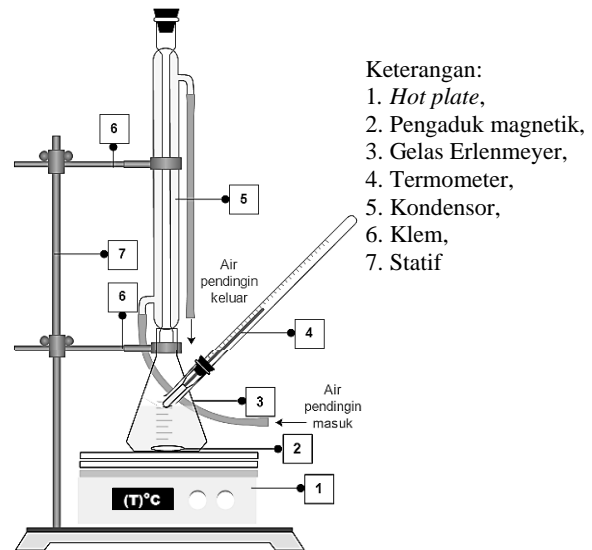
Gambar 1. Skema peralatan proses swelling
