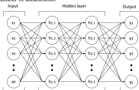
Figure 1. VSM-NN Topology.
