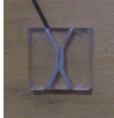
Figure 3. Fabricated directional coupler images.
