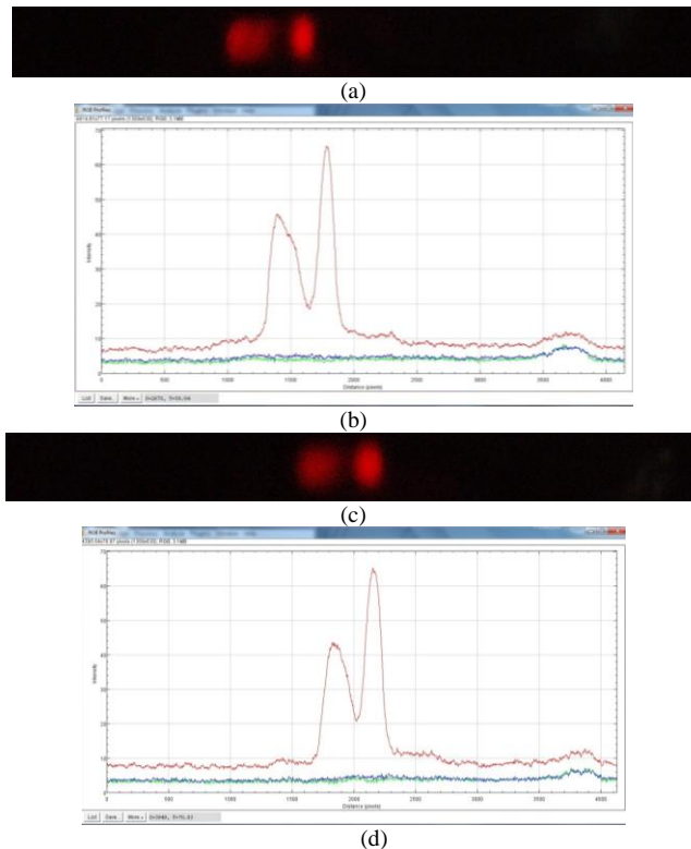
Figure 5. Directional coupler waveguide with 5 mm coupling length with input B1 (a) B2 B2 port (b) RGB B2 A2 port plot (c) A1 B1 port (d) RGB port A1 B1 plot.
