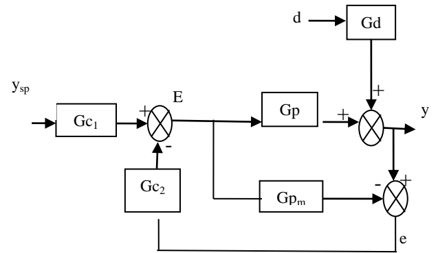
Figure 4. The structure of 2DOF-IMC standard
