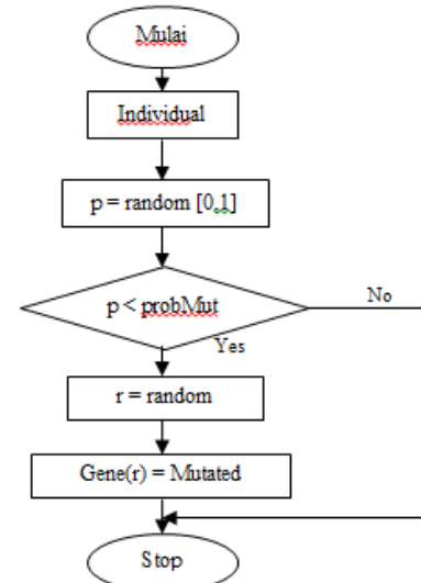
Figure 5. Flowchart of Mutation
