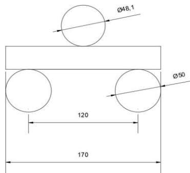
Figure 7. The layout of the experiment (mm).
