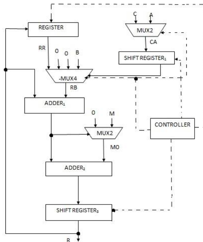
Figure 3. Montgomery Multiplier
