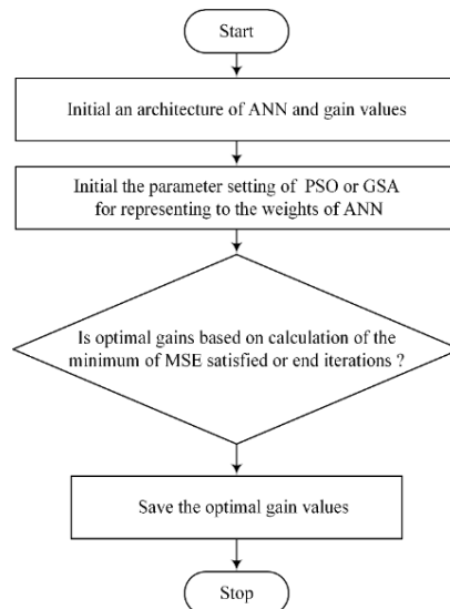
Figure 3. Steps of hybrid methods for finding optimal gains
