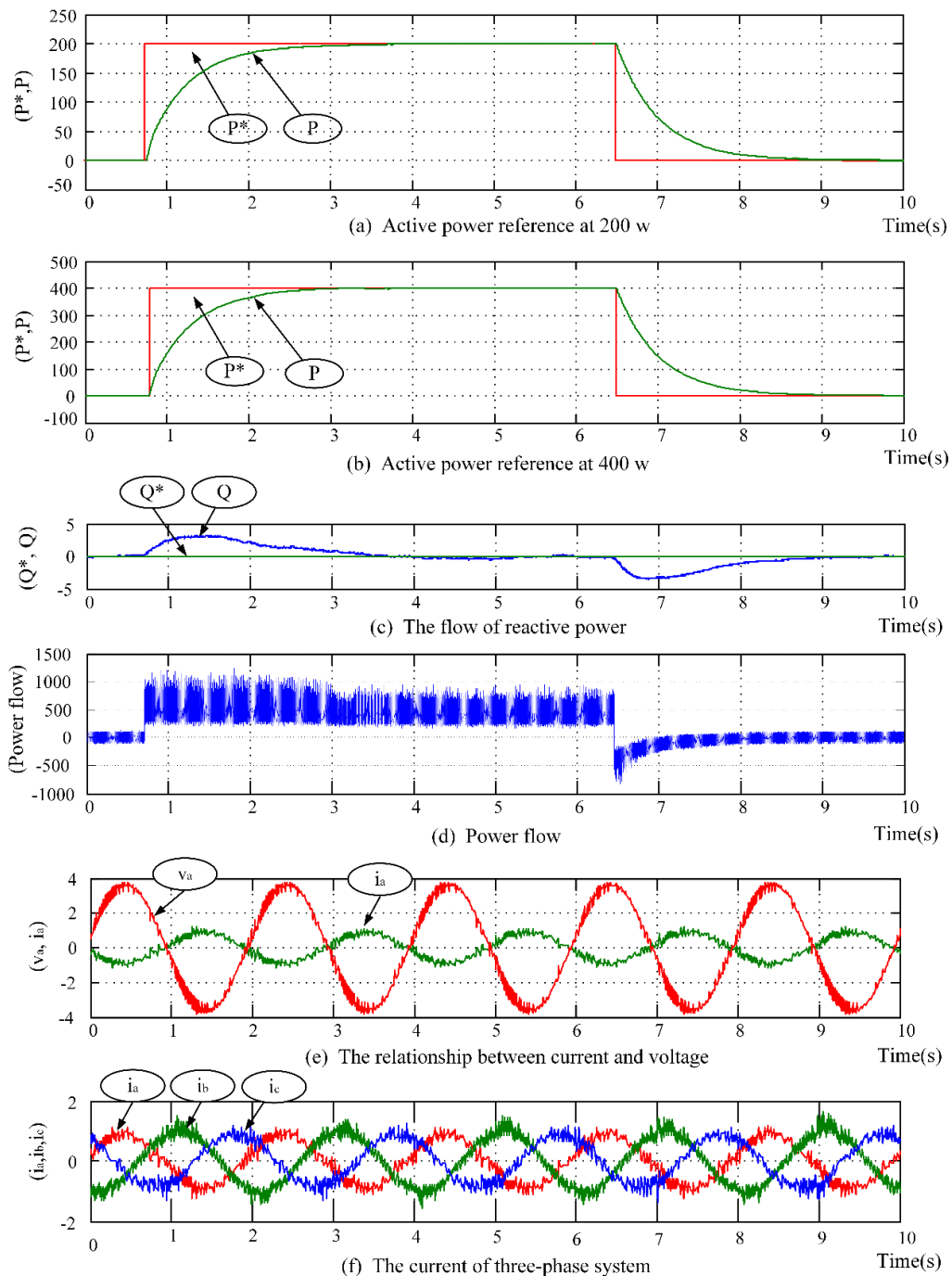
Figure 10. Step change of active power reference at 200 w to 400 w tuning gains by PSO-ANN
