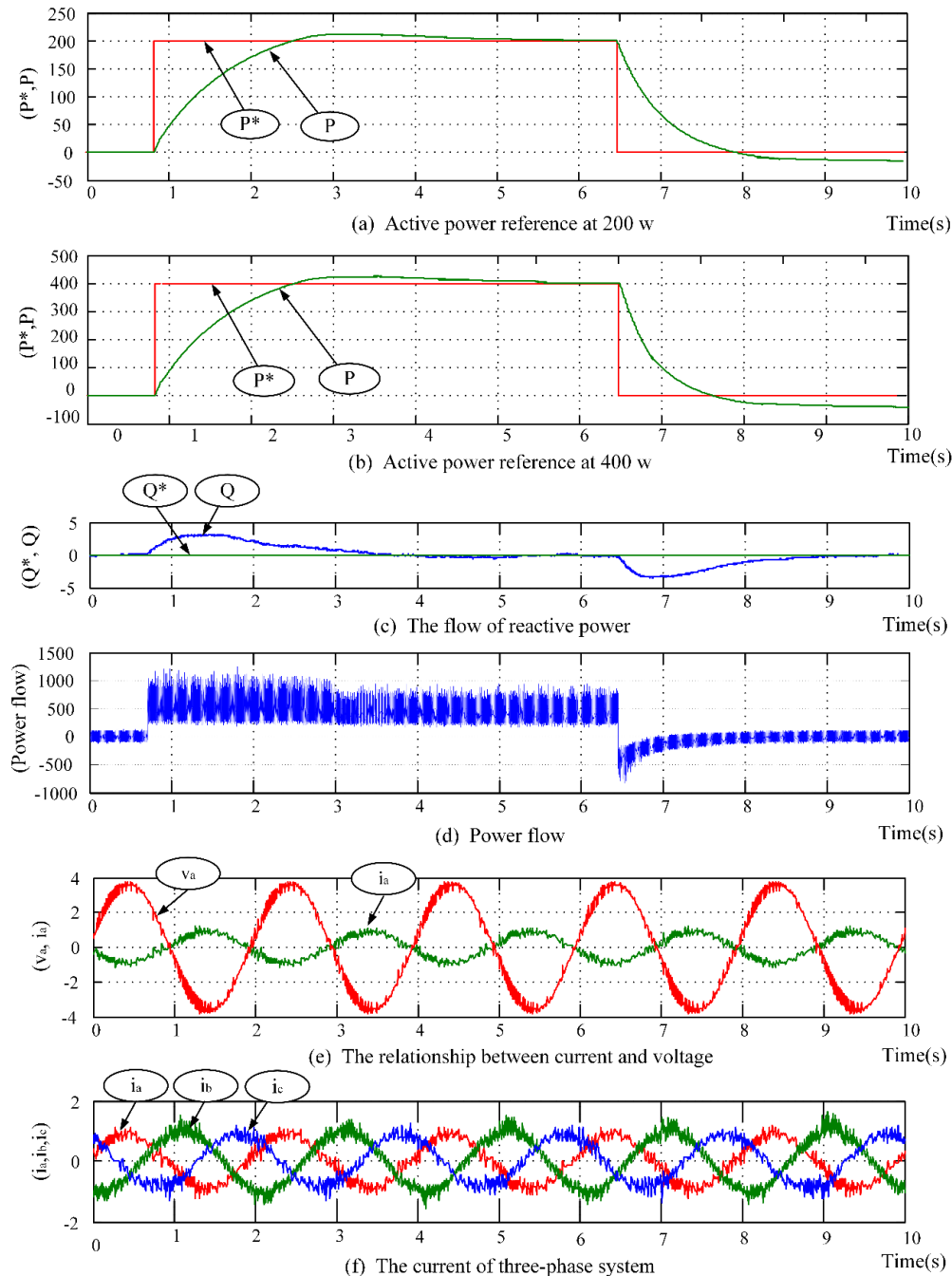
Figure 11. Step change of active power reference at 200 w and 400 w tuning gains by GSA-ANN
