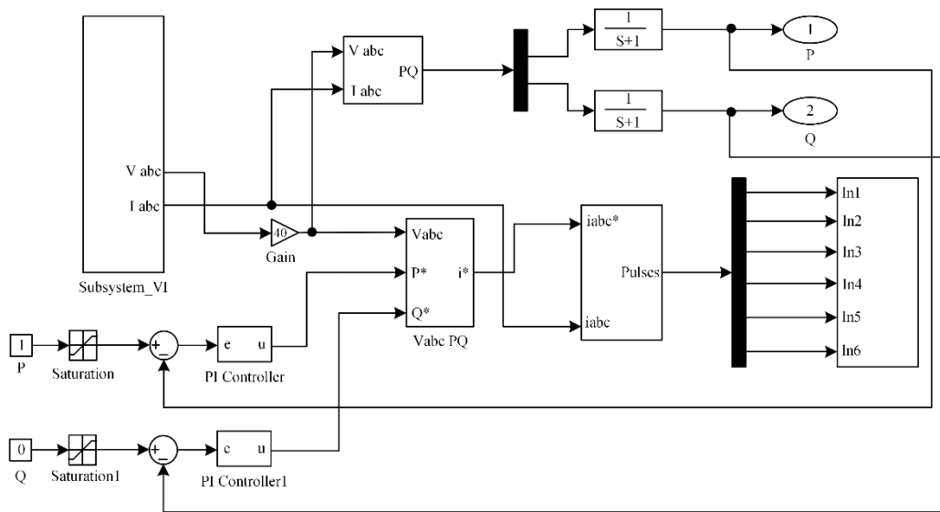
Figure 6. Simulink diagram
