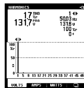
(b) THDV at step 0-400 w
