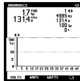
(b) THDV at step 0-200 w
