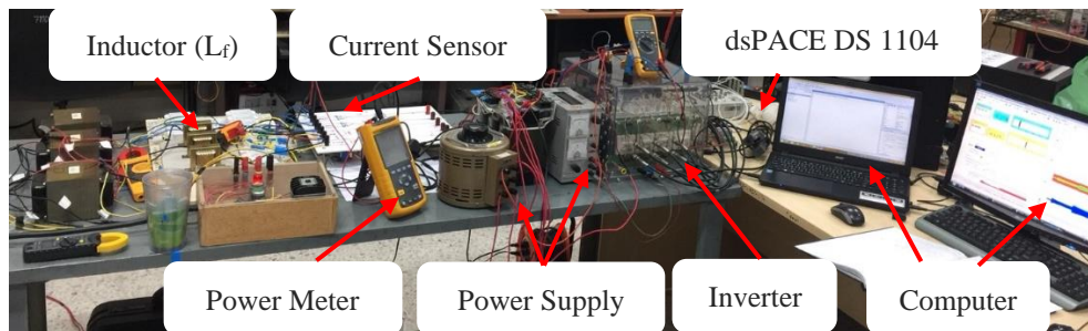
Figure 4. The power flow control system
