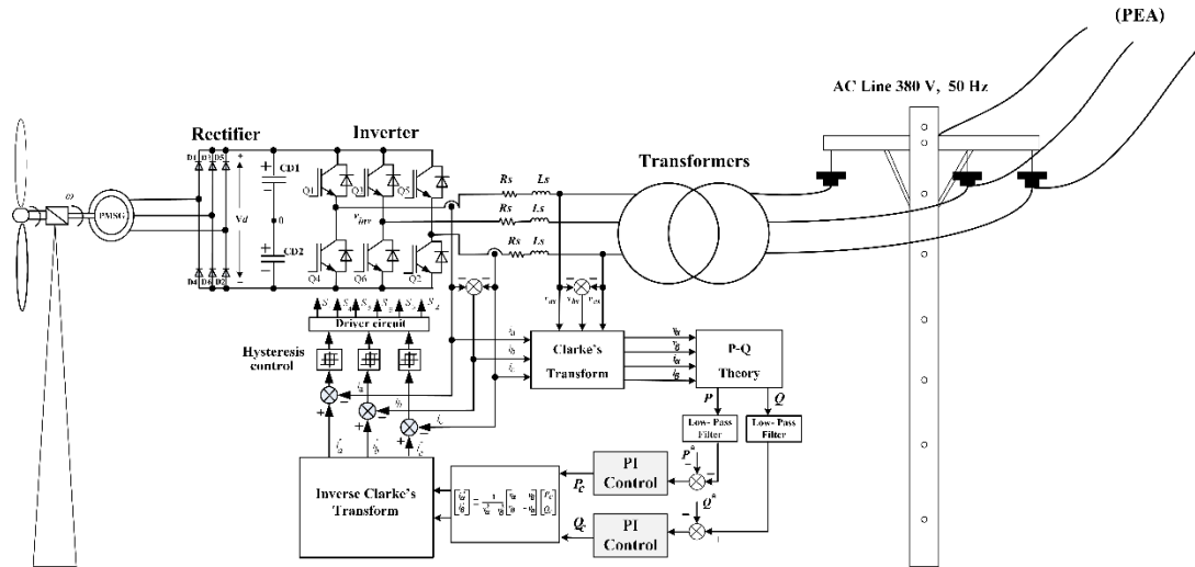
Figure 1. Scheme of wind turbine based on PMSG generator connected to the grid system
