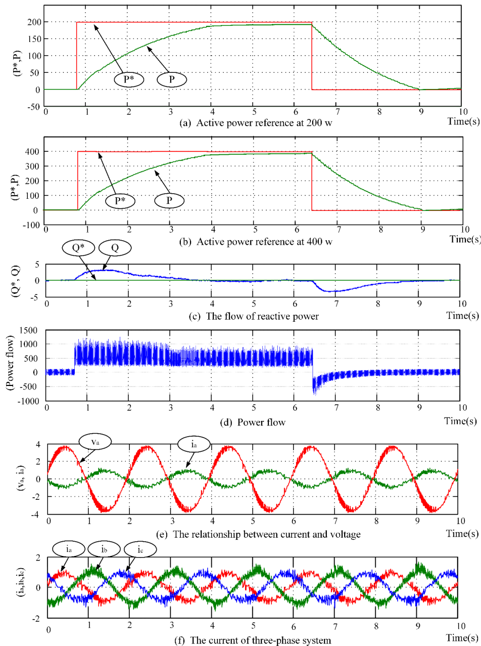
Figure 8. Step change of active power reference at 200 w to 400 w tuning gains by PSO
