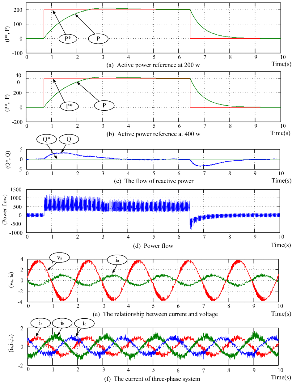
Figure 7. Step change of active power reference at 200 w to 400 w tuning gains by the pole placement
