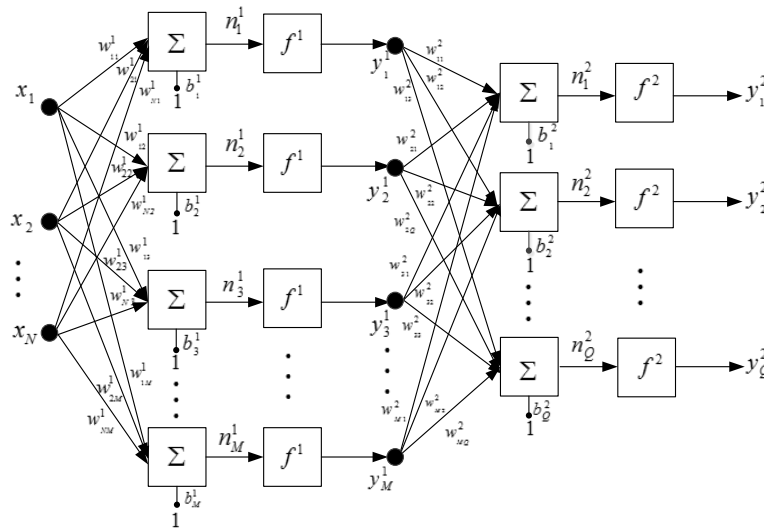
Figure 2. The architecture of ANN [26]
