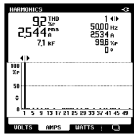
(a) THDi at step 0-200 w
