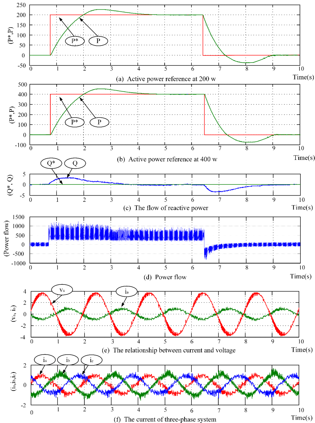
Figure 9. Step change of active power reference at 200 w to 400 w tuning gains by GSA
