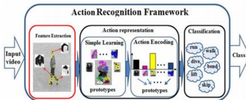
Figure 1. Action recognition framework [3]
