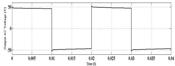
Figure 8: 1- \Phi , Output AC voltage of diode-clamped inverter
