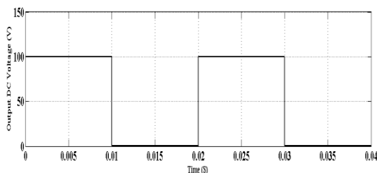
Figure 7: 1- \Phi , Output DC voltage of diode-clamped inverter
