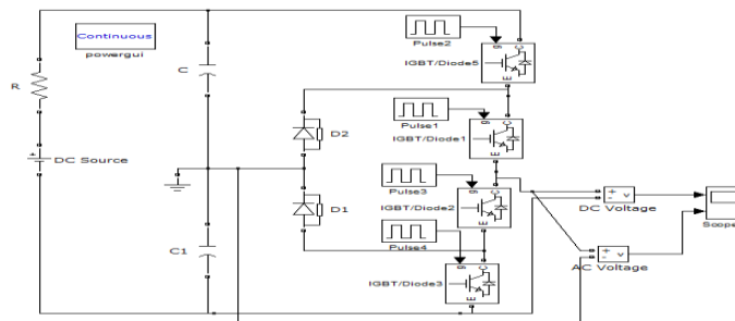
Figure 6: Simulated circuit diagram for 1- \phi , diode-clamped inverter
