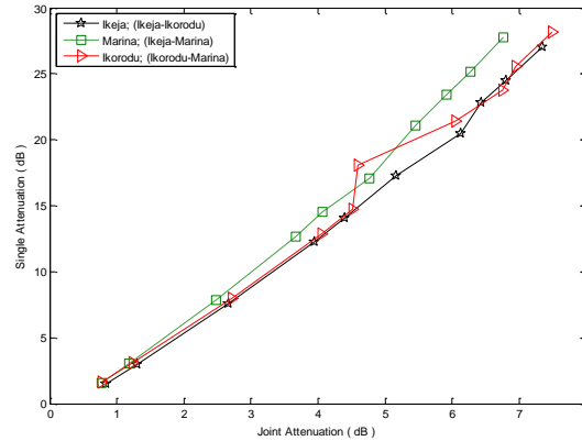
Figure 8. CDFs of single site attenuation site against joint attenuation
