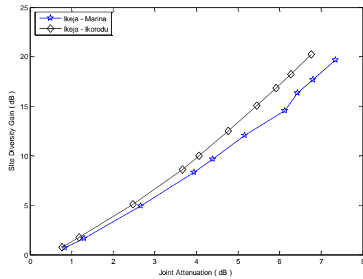
Figure 6. Site diversity gain versus joint attenuation
