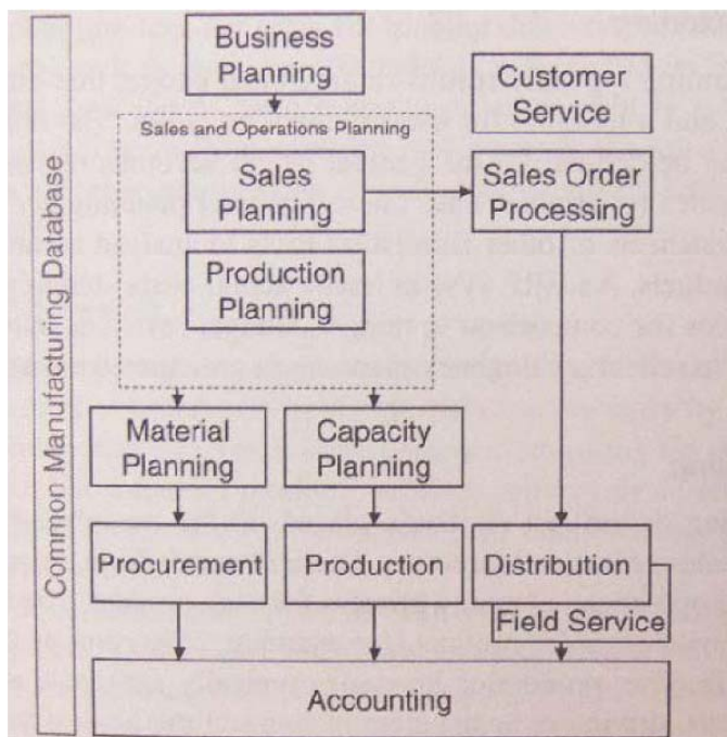
Figure 1 - Architecture of an ERP System
