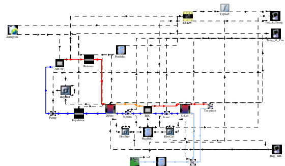
Fig. 2 Simplified trnsys simulation
