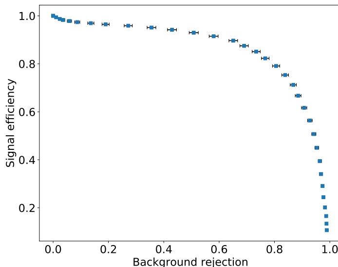
Figure 10. Signal efficiency as a function of background rejection, varying the required minimum energy of the blob candidate 2 between 0 and 500 keV, in the \beta\beta 0\nu region.
