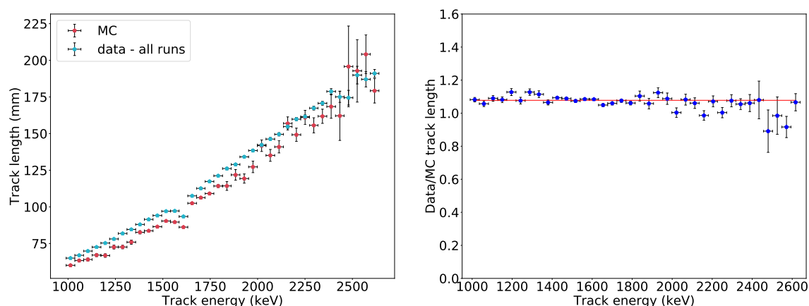
Figure 6. Track length as a function of the track energy for data and Monte Carlo. The left panel shows the average value for each bin, while the right panel shows the ratio between data and Monte Carlo and a linear fit to the distribution.
