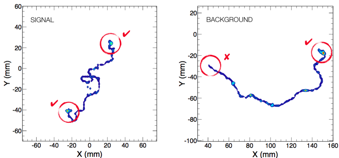
Figure 1. A \beta\beta\nu event (left) and a single electron background event from a 2.447 MeV ^{214}\text{Bi} gamma (right) in Monte Carlo simulation. Both events are simulated in gaseous xenon at 15 bar gas pressure.
