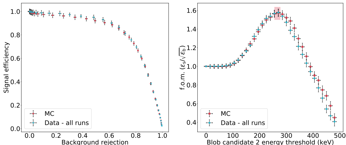
Figure 9. Left: signal efficiency as a function of background rejection (proportion of background events removed from the sample by the blob cut), varying the required minimum energy of the blob candidate 2 . Right: figure of merit (defined in eq. 4.1) as a function of the threshold on the energy of the blob candidate 2 after rescaling Monte Carlo. The highlighted area corresponds to the best threshold. In both figures, data and Monte Carlo simulation are shown.
