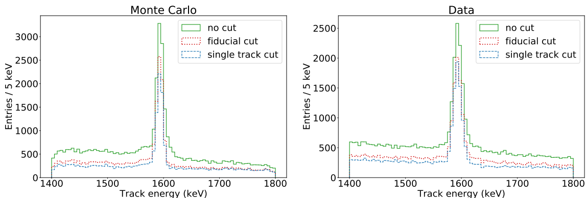
Figure 3. Distribution of the track energy in the region around the double escape peak before any cut and after the single-track and the fiducial cut (see text for details). Left: Monte Carlo, right: data.
