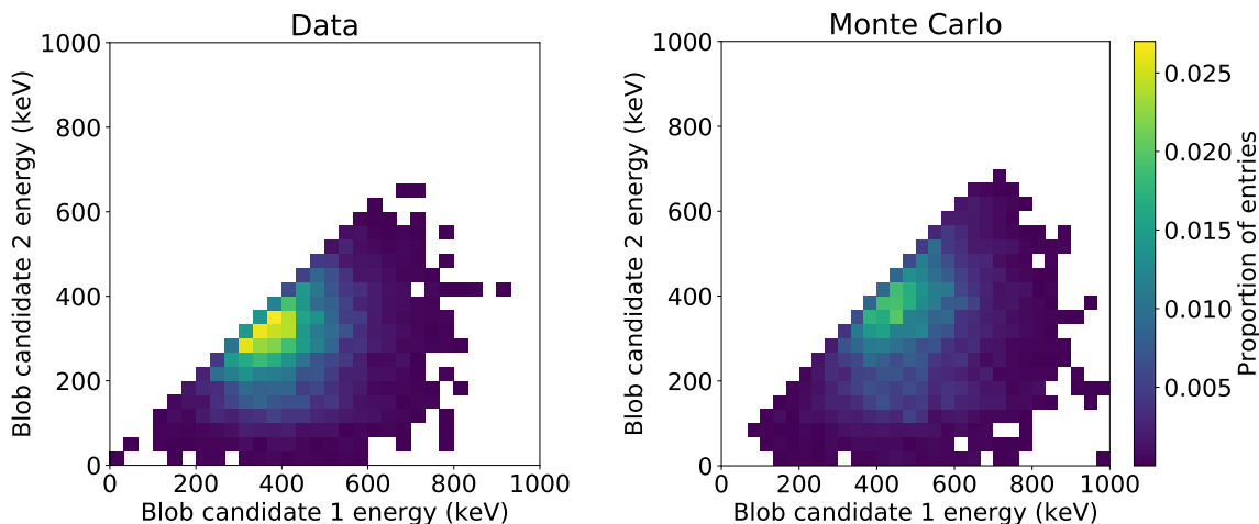
Figure 4. Distribution of the energies of blob candidate 1 and blob candidate 2 for data (left) and Monte Carlo (right), in the 1570–1615 keV region, under the ^{208}\text{Tl} double escape peak.
