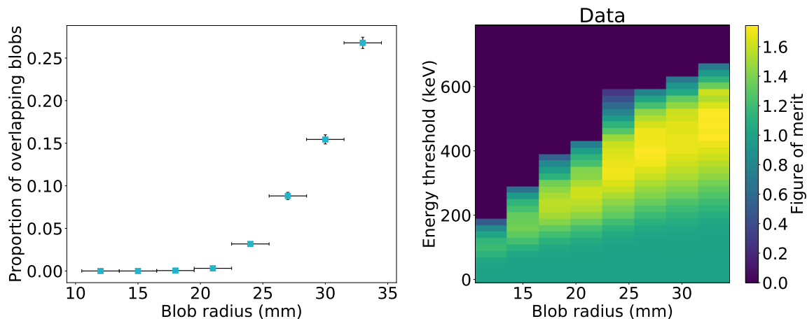
Figure 11. Proportion of events with overlapping blob candidates (left) and dependence of the figure of merit on the blob radius and the energy threshold on the blob candidate 2 (right).
