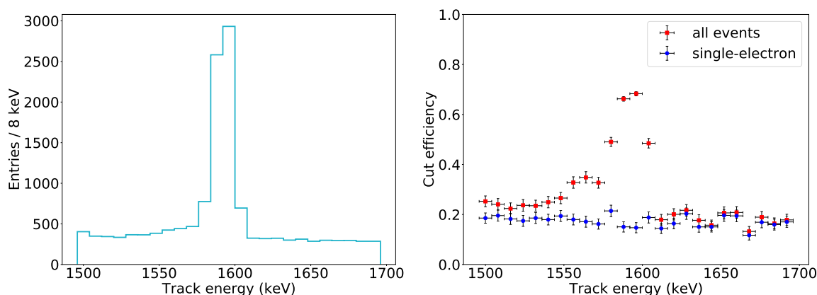
Figure 7. Blob cut efficiency for Monte Carlo, using the full event sample and a sample of single-electron events. The histogram on the left side represents the full sample of track energies and the plot on the right side shows the fraction of the total number of events passing the cuts for each one of the two samples.
