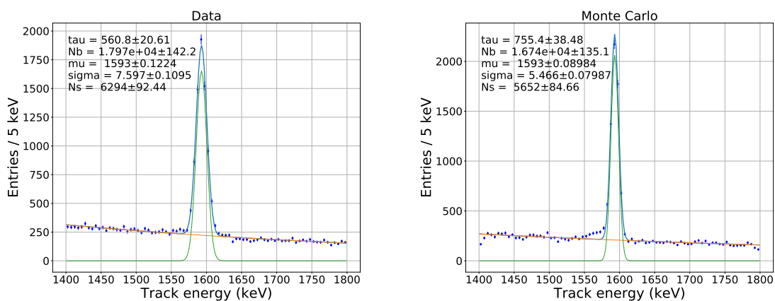
Figure 8. Energy spectrum and results of the gaussian+exponential fit for both data (left) and Monte Carlo (right).
