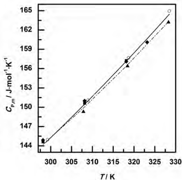
FIGURE 3. (a) Isobaric molar heat capacity for propan-1-ol: this work (—); polynomial of Zábranský et al. [37] (—•—); Counsell et al. [38] (▲); van Miltenburg et al. [39] (○); Comelli et al. [40] (◆); Peleteiro et al. [41] (■).
