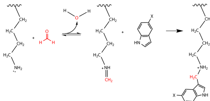
Figure 11: Indole conjugation to an amino acid with formaldehyde as reagent [11]
