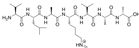
Figure 35: Peptide with formaldehyde
