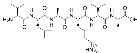
Figure 34: Peptide without alanine with formaldehyde
