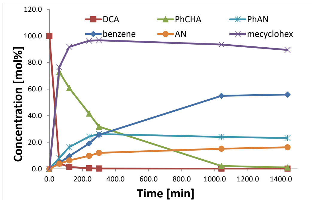
Figure 8. Dehydrogenation of DCA on Pd/C at different times. Reaction was carried out at 200°C on different times. That allow us to regard the kinetic aspect of the dehydrogenation step on the reference catalyst. Species concentrations relatives to mol %. It can be observed that in the first hour almost all the DCA has been transformed into PhCHA. At five hours PhAN reaches a maximum since where its concentration starts to decrease. Finally, Pd/C also cleavages the substrate into aniline and benzene, but in much less quantity than Pt/C (.). It can be appreciate the third order kinetics DCA PhCHA BZ+PhAN+AN. As an anecdote methylcyclohexane concentration has been included, showing somehow the solvent bias the activity on the catalyst surface.
