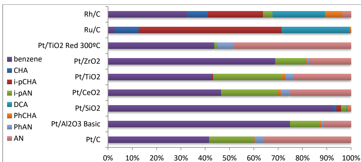
Figure 12. Rh/C, Ru/C and several Pt catalysts dehydrogenation of i-pCHA. Normalized concentrations. All the reactions were carried on at 180 °C during 180 mins. Rh/C and Ru/C are not very active, neither selective. Rh/C seem to be a very good catalyst towards the DCA formation. Pt catalysts show high activity, but not selectivity on the working conditions. CeO or TiO 2 showed some activity towards the dehydrogenated product but also towards aniline and benzene formation, information which says us some i-propylamine has been also formed. Pt/SiO 2 will turn into an important catalysts in case some N-substituted aniline became the fountain of benzene all around the world. Pt/C presented some activity towards the dehydrogenated product, but mostly catalyzes the cleavage of the amine, something to be avoided.
