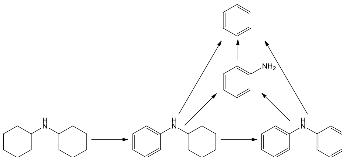
Scheme 7. Schematic for the reaction network for the side-product formation from DCA dehydrogenation
