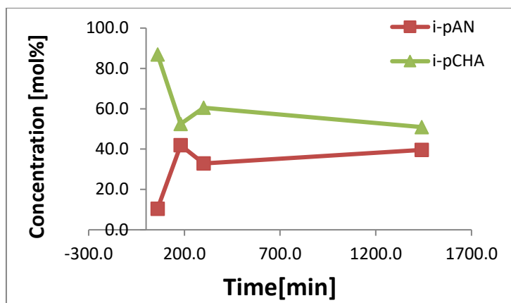
Figure 15. Kinetics of the dehydrogenation of i -pCHA at 200°C on Pd/BaSO 4 . It can be seen an strange slope for the second and third point, consequence of the experimental mistake. Anyways, the last point shows the thermodynamic of the reaction, and can be interpreted that the catalyst get poisoned at some point. The other compounds haven't been showed due to they don't get over 2.2% in any case.
