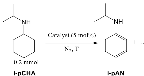
Scheme 8. Schematic for the dehydrogenation of iso-propylcyclohexylamine.
