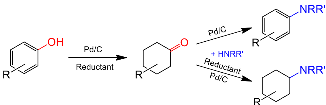
Scheme2. Phenol amination with cyclohexanone as intermediate.
