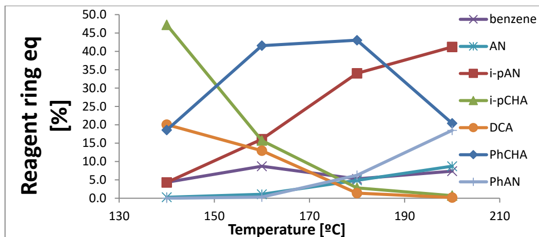
Figure 9. Percentages of the different obtained products are expressed toward rings equivalent of the initial i-pCHA. Pd/C is the catalyst. Reactions have a duration of 180 min. The graph shows similarities with the DCA dehydrogenation (Figure 6). It can be regarded that higher temperatures present the better selectivity, but from the hand of a crescent cleaving activity.
