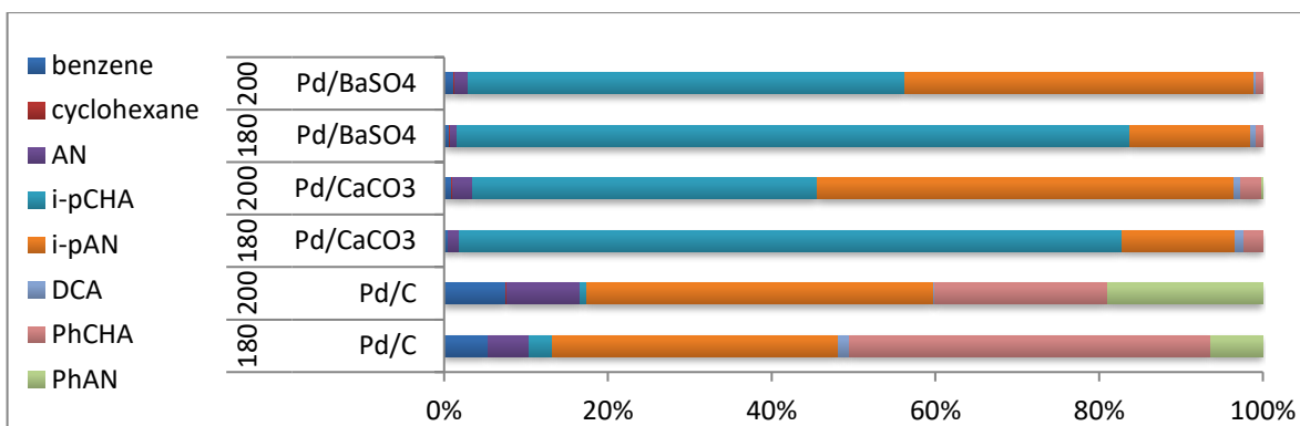
Figure 13. Dehydrogenation of i -pCHA carried out by Pd catalysts. Reaction time was fixed on 180 min. A new temperature was tested (200°C) in order to compare the reaction yield with previous obtained data of the same reaction at lower temperature (Figure 11). Correspondent temperature is written down in the column to the left of the catalyst name. As it can be seen, the selectivity has been maintained on a satisfactory way rising the temperature, also the transformation has been increased. Pd/CaCO 3 and Pd/BaSO 4 raised its activity towards the desired product with the temperature, which means that with longer times, higher dehydrogenation will be achieved (Figure 14)(Figure 15).
