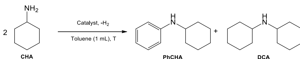
Scheme 4. Reaction of two CHA molecules towards PhCHA and DCA
