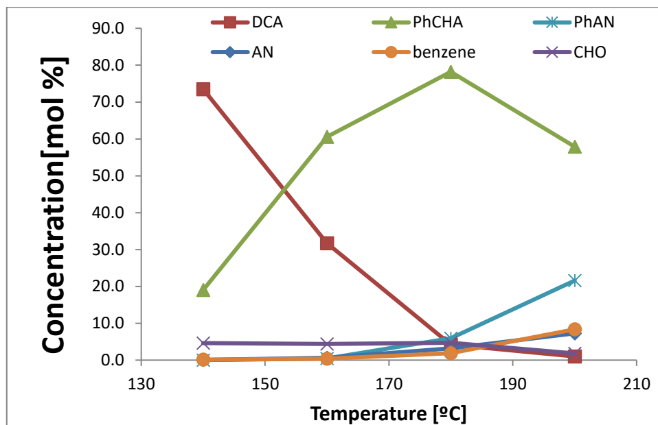
Figure 6. Dehydrogenation of DCA after 180 min of reaction using Pd/C as catalyst. CHA isn't displayed due to its small concentration in all the experiments.
