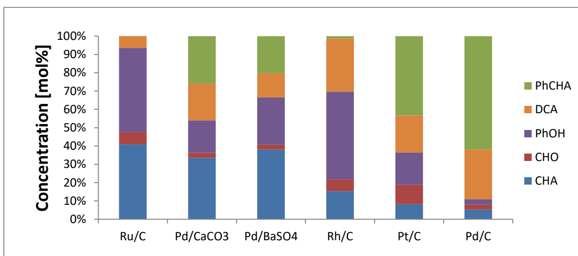
Figure 3. Normalized concentration of the different products after reaction at low hydrogen pressures (0.125 bar) for 300 min at 140 °C.
