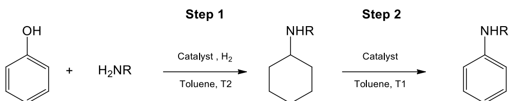
Scheme 5. Schematic of the two-step-one-pot approach.
