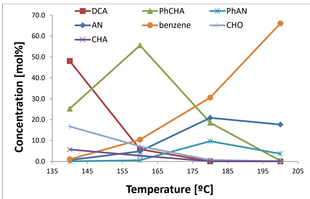
Figure 7. Dehydrogenation of DCA after 180 min of reaction using Pt/C as catalyst. CHA isn't displayed due to its small concentration in all the experiments.
