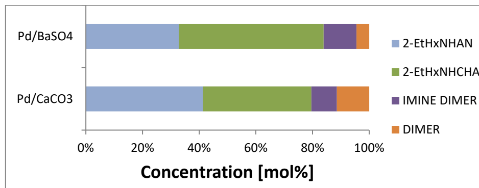
Figure 16. Relative concentrations of the products obtained the reaction between 1 eq. of PhOH and 1.4 eq. of 2-ethyl-1-hexylamine (2-EtHxNH). The percentages of the reagents have been taken into account as 100 % for the PhOH and an additional 140 % for the amine. The reaction was catalyzed with Pd/BaSO 4 and Pd/CaCO 3 respectively. H 2 was used as reductant at the pressure of 0.125 bar. Reactions were carried out at 140°C during 300 mins. It hasn't been showed respective reagents concentration in the graph in order to make more visible the different products proportion, due to not much transformation was achieved: 25.6 % and 40.6 % (from 100%) transformation was reached for phenol, respectively, whereas 25.8 % and 46.4 % (from 140 %) transformation was reached for the amine.
