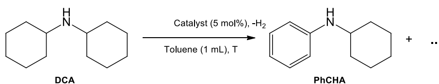
Scheme 6. Dehydrogenation of dicyclohexylamine
