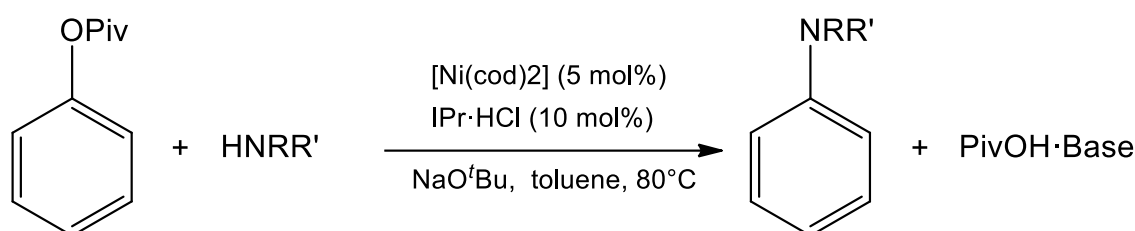
Scheme1. Conversion of phenylpivalates to anilines 8 .
