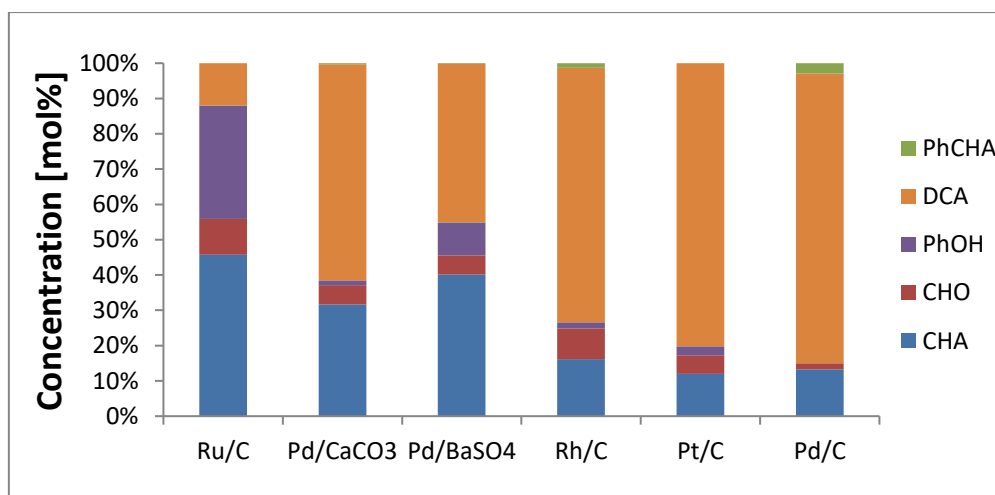
Figure 4. Normalized concentration of the different products after reaction at high hydrogen pressures (2 bar) for 60 min at 140 °C.
