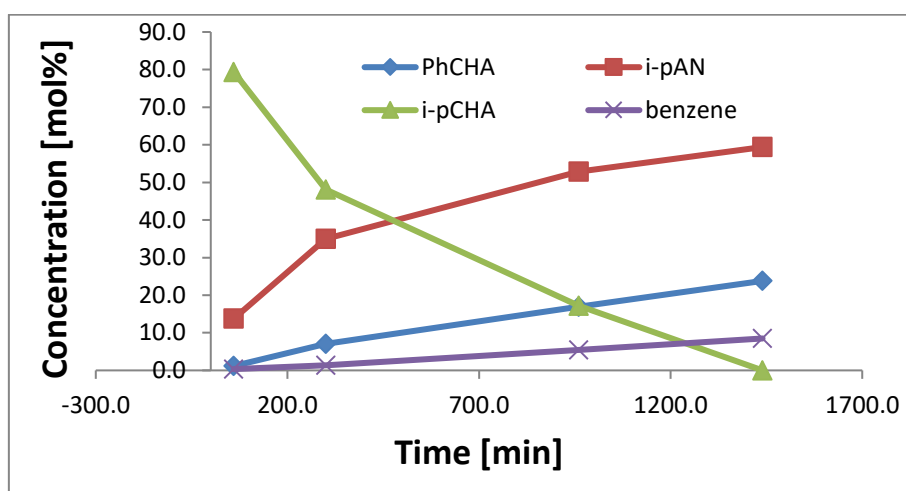
Figure 14. Kinetics of the dehydrogenation of i-pCHA at 200°C on Pd/CaCO 3 . As it can be seen, the longer the time of reaction, the more products are obtained, predominantly the dehydrogenation one. Rest of the compounds haven't been showed because they weren't superior to 3 % in any case.
