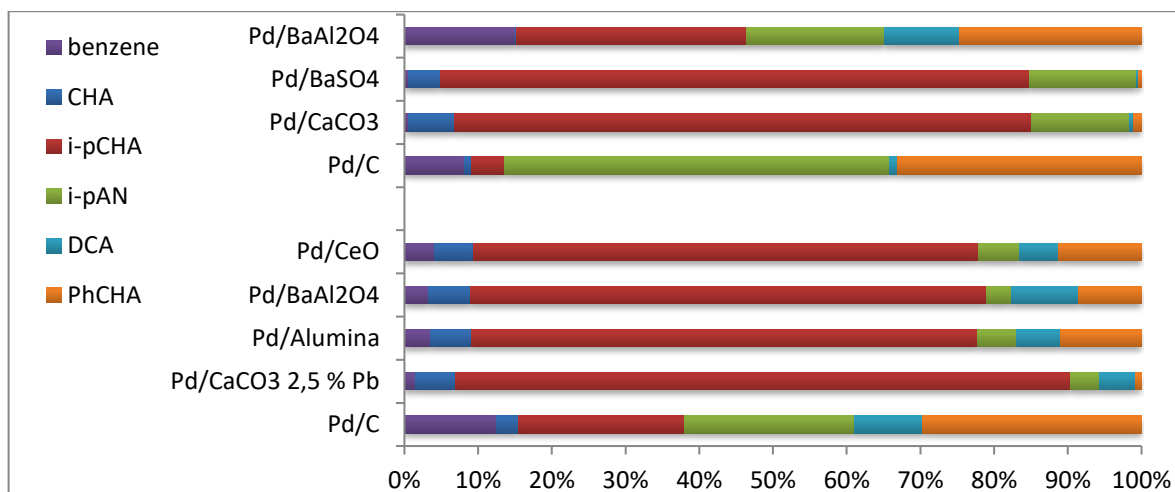
Figure 11. Concentration of iso-propylcyclohexylamine (i-pCHA) dehydrogenation products. Reaction was carried out with different Palladium catalysts during 180 min. First group of reaction was performed at 180°C. The reactions in the lower block were performed at 160°C
