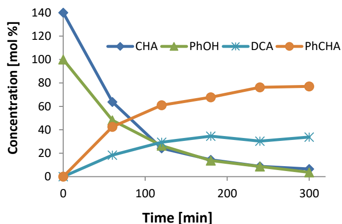
Figure 2. Amination of phenol with CHA at 0.125 H 2 bar and 140 °C (left) and the same reaction at 2 bar H 2 (right).
