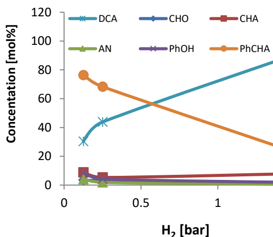
Figure 1. Concentrations of the reaction of phenol with cyclohexylamine in the presence of hydrogen after 240 minutes of reaction at different hydrogen pressures. The reaction was carried out at 140 °C. It can be clearly observed that at high pressures the hydrogenated Dicyclohexylamine product is obtained as main product.
