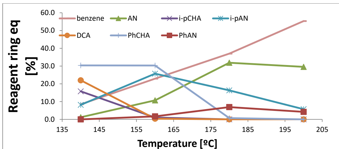
Figure 10. Reagent ring equivalents (%) of the different obtained products on the dehydrogenation of i -pCHA with Pt/C as a catalyst. Reactions were stopped after a course of 180 min. Graph is very similar to the DCA dehydrogenation (Figure 7). It can clearly be seen the high cleavage activity in every temperature, but the highest yield towards the dehydrogenated product was found at 160°C.
