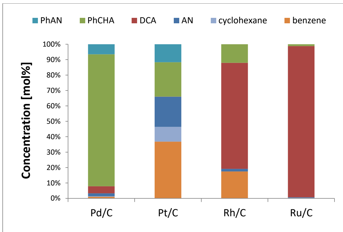
Figure 5. Concentration of the different products of the dehydrogenation of DCA and DCA itself after 180 min. Reactions were carried out at 180 °C using different carbon supported catalysts.
