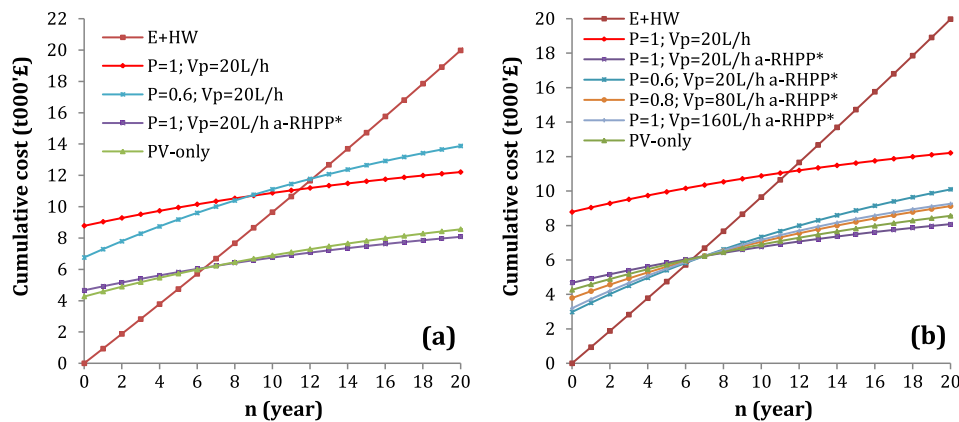
Fig. 14. Comparison of the cumulative costs of the different PVT configurations studied to that of the PV-only system with a discount rate of d = 0.08 , as well as to that of the conventional scenario (electricity + hot water costs (squares)) with a discount rate of d_c = 0.025 and an inflation rate of i = 0.032 , when the optimum augmented Renewable Heat Premium Payment (a-RHPP*) is given as one-off voucher at the beginning of a system's lifetime.
