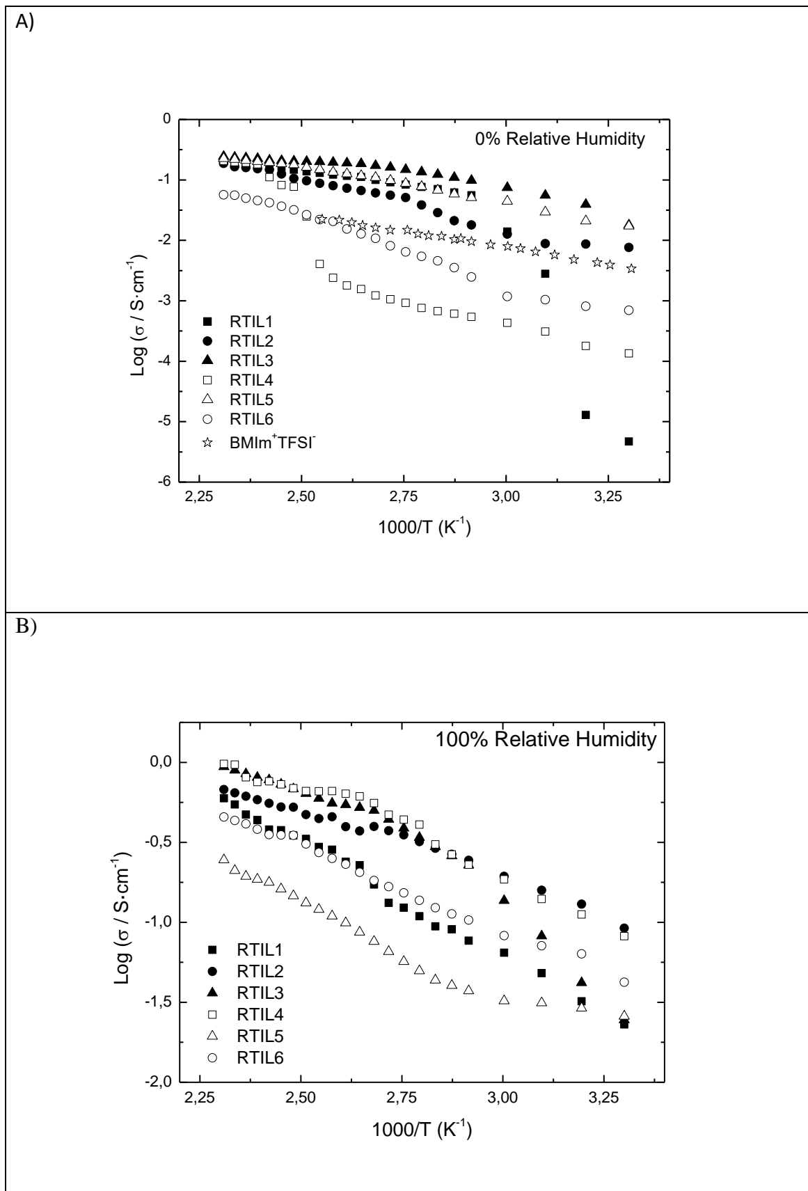
Figure 1. Arrhenius Plot of ion conductivity data of the selected RTILs for this study: A) dry conditions ( \text{BMIm}^+\text{TFSI}^- data adapted from Ref. 40); B) saturated conditions.
