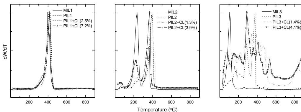
Figure 3. Differential TGA curves of the three families of PILs as a function of the crosslinker molar percentage, showing their varying thermal stabilities. The corresponding monomer derivatives are also depicted for comparison.
