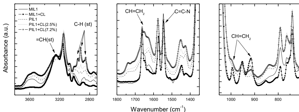
Figure 4. FTIR spectra of poly[1-(3H-imidazolium)ethylene] bis(trifluoromethanesulfonyl)imide (PIL1) samples as a function of the crosslinker molar percentage. The starting 1-H-3-vinylimidazolium bis(trifluoromethanesulfonyl)imide monomer is included as reference.
