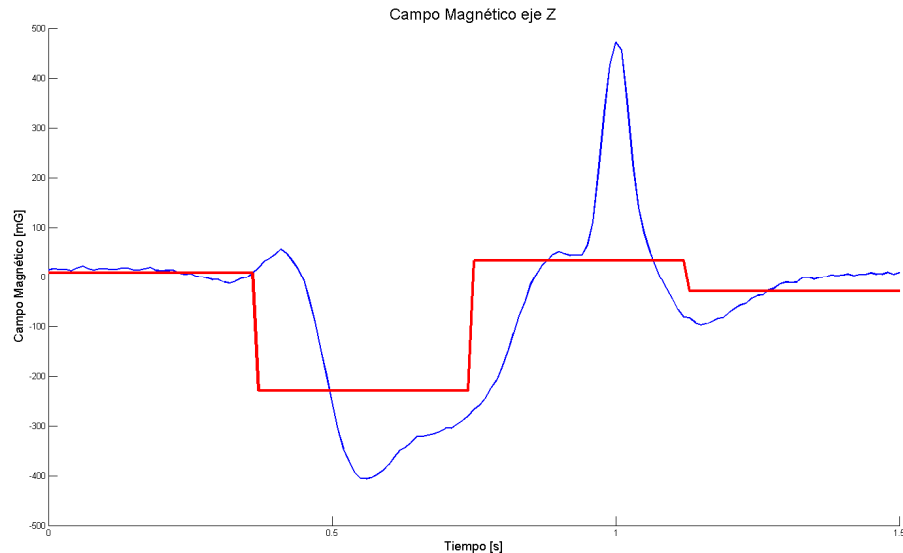
Fig. 22 Average-Bar Transform
