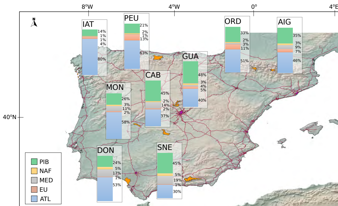
Figure 4: Proportion of air mass transport scenarios over NP in mainland Spain based on clustering 48-h back-trajectories at surface level in the period 2008-2012
