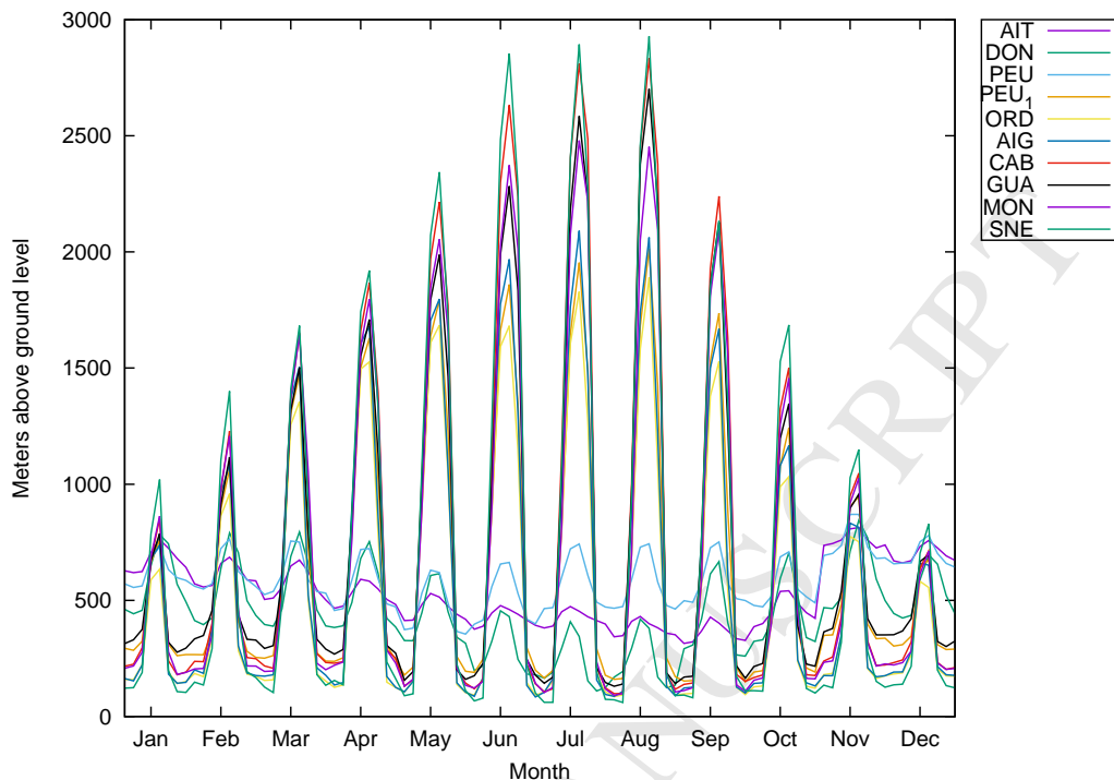
Figure 6: Mean daily cycles of the PBL height for each month in NP of Spain during the period 2008-2012
