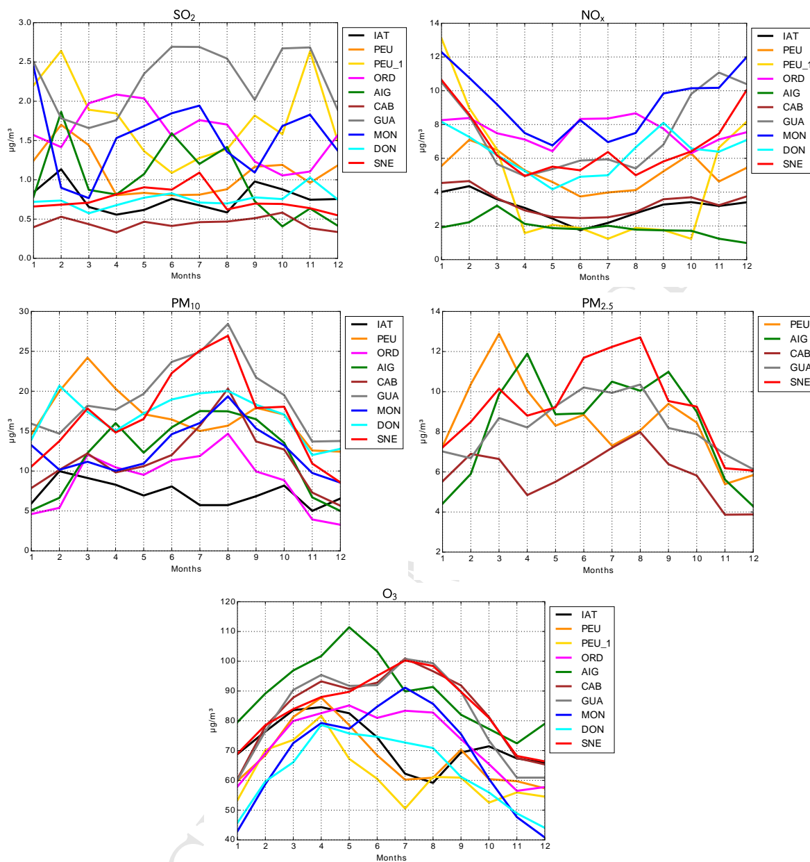
Figure 5: Monthly mean concentrations of atmospheric pollutants in NP of mainland Spain for the period 2008-2012
