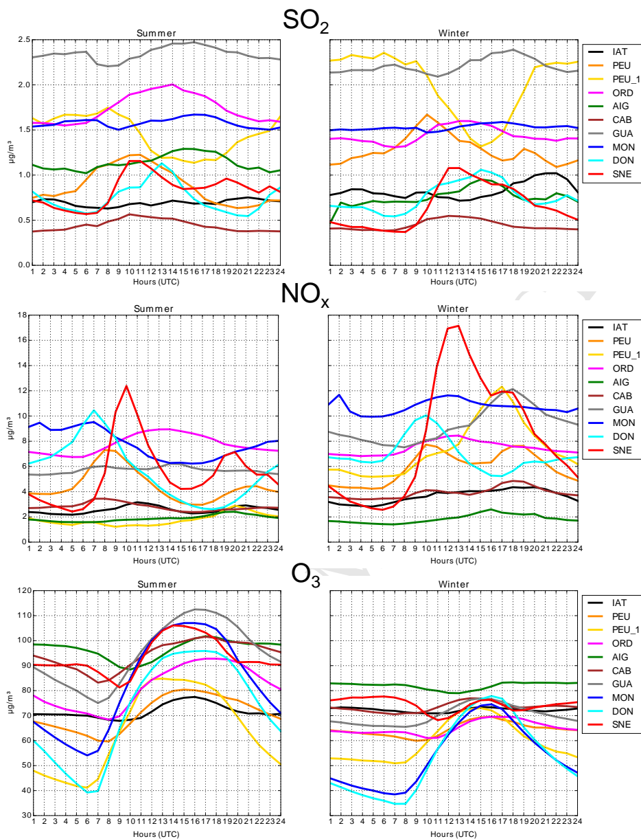
Figure 8: Winter and summer mean daily cycles of the concentrations of gaseous pollutants in NP of Spain for the period 2008-2012
