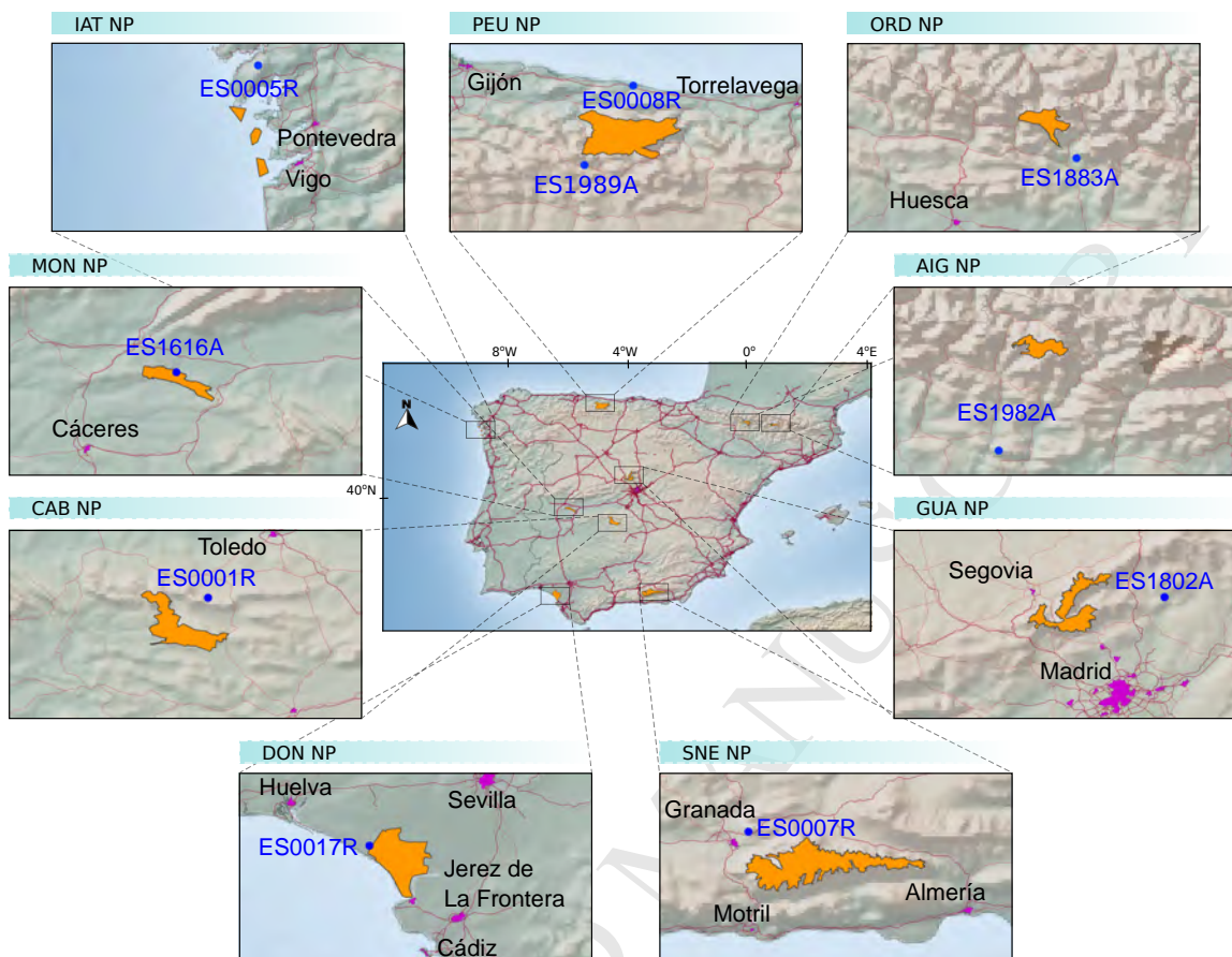
Figure 1: Location of the NP and the monitoring stations used in this study.
