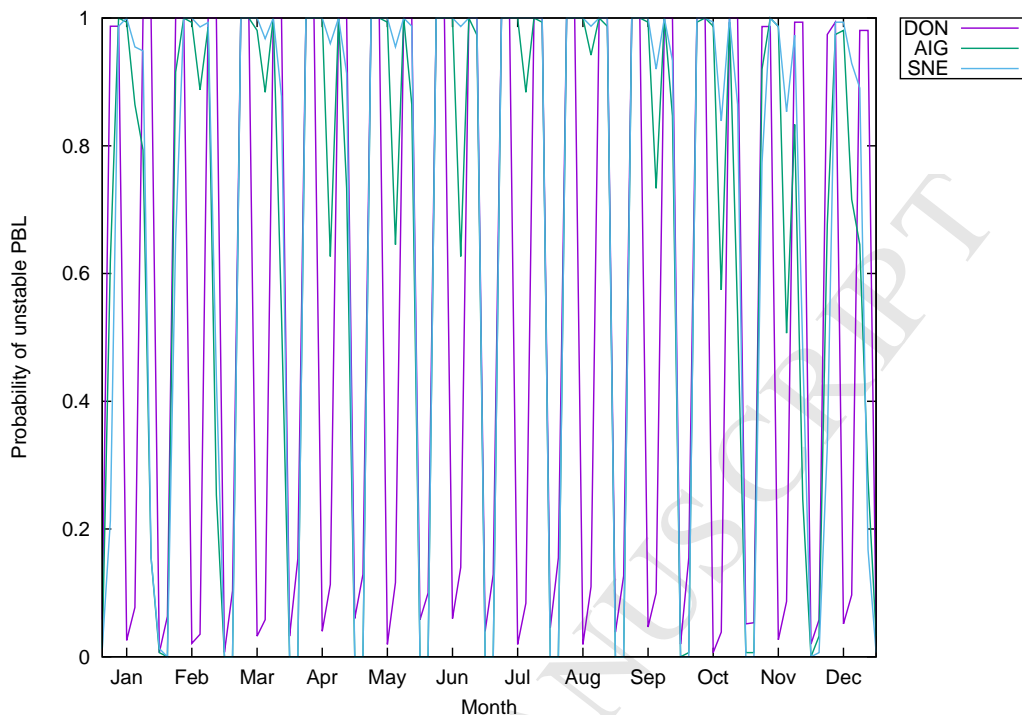
Figure 7: Mean daily cycles of the probability that the PBL be unstable for DON, AIG and SNE during the period 2008-2012.
