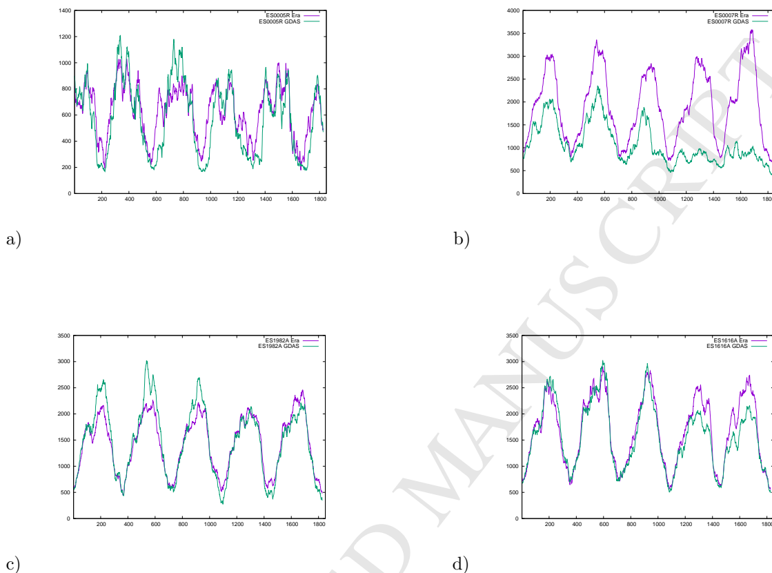
Figure 2: Number of days since Jan 1st 2008 in the X axis versus moving average of PBL height at 15:00 UTC, Y axis, in four locations: a) DON, b) SNE, c) AIG and d) MON. The reported value of PBL height is a simple mean of the actual values during the 29 days centered around the considered date, at 15:00 UTC every day. ERA-Interim values versus GDAS ones.
