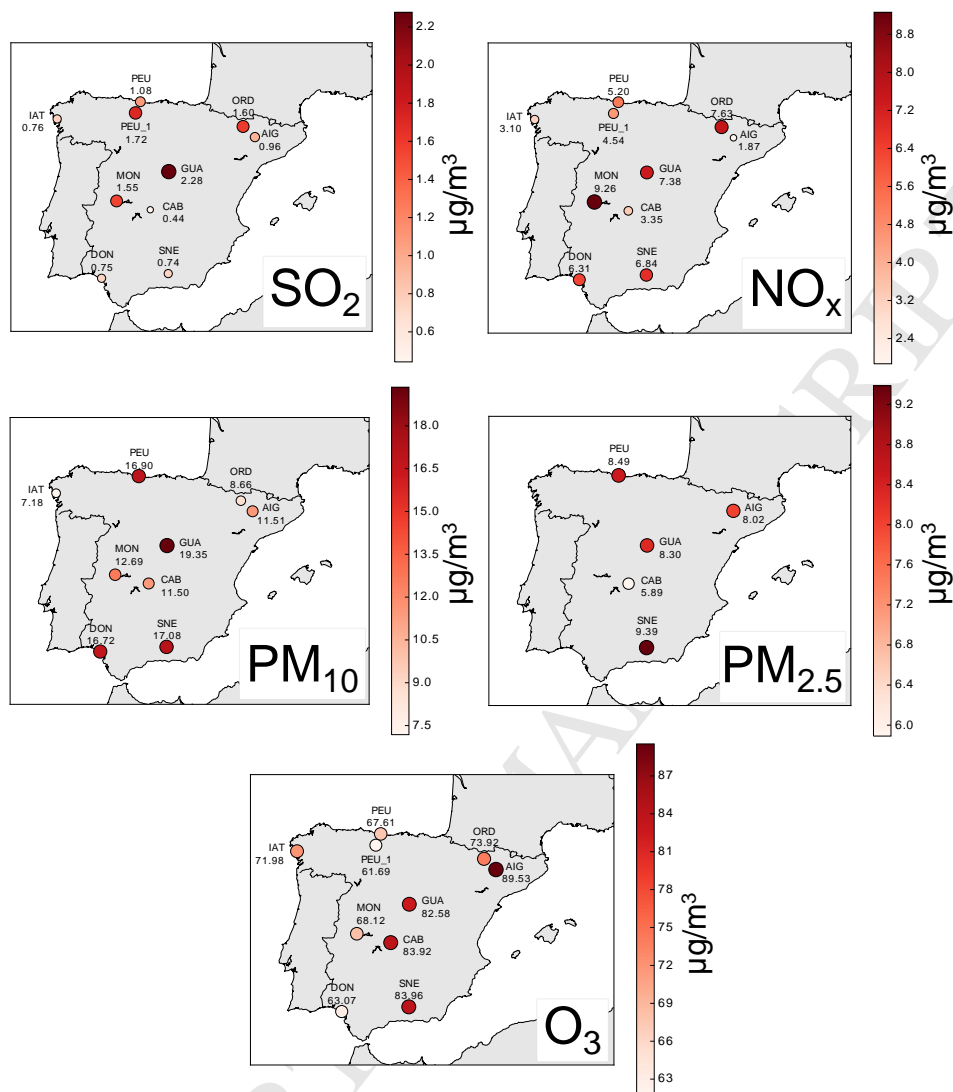
Figure 3: Average levels of atmospheric pollutants in NP of mainland Spain for the period 2008-2012
