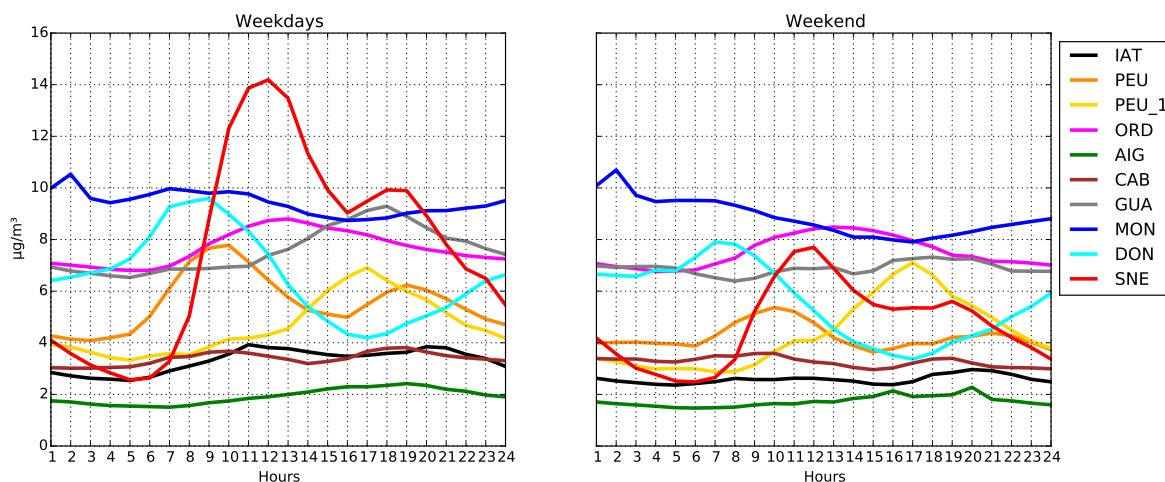
Figure 9: Weekdays and weekends mean daily cycles of NO_x concentrations in National parks of Spain for the period 2008-2012
