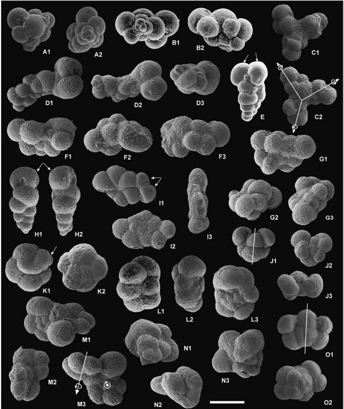
FIGURE 6. Examples of extreme aberrant forms of early Danian planktic foraminifera. Scale bar, 100 microns. A and B, Guembeltria spp., multiple ultimate chambers (racemiguembeliform multiserial test). C, Guembeltria sp. (probably G. cretacea ), attached triplets (triamese). D, Guembeltria sp. or Woodringina sp., general monstrosity (probably attached twins with abnormal, kummerform, and protuberant chambers). E, W. hornerstownensis , double or twinned ultimate chambers. F, Guembeltria sp. or Woodringina sp., general monstrosity (probably attached twins with abnormal chambers). G, Parvularugoglobigerina sp. or Palaeoglobigerina sp., general monstrosity. H, W. hornerstownensis , last chamber in anomalous position, with test going from biserial to uniserial. I, Pv. longiapertura , additional chambers and apertures. J, Palaeoglobigerina sp. (probably Pg. luterbacheri ), attached twins (Siamese). K, Pv. sabina , bulla-like ultimate chamber. L, Pv. eugubina , twisting of entire test (extreme kinking) and overdeveloped last chambers. M, Parvularugoglobigerina sp. (probably Pv. longiapertura ), two specimens with fused tests. N, Palaeoglobigerina sp., general monstrosity. O, Parvularugoglobigerina sp.; additional chambers and apertures. All specimens come from El Kef, except for some from Ain Settara (E, F).
