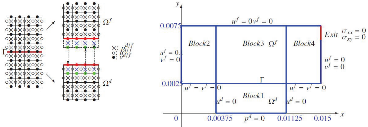
FIGURE 1. (Left) Communications between two partitioned subgrids. (Right) Geometry of the cross-flow membrane filtration model.
