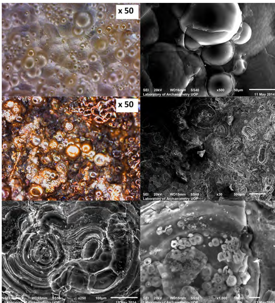
Figure 8 FOM and SEM images of the iridescent (up) and the brown layer (middle and down) of the plant-ash sample.
