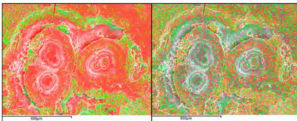
Figure 9 Mapping of the concentration of Si, Mn and Fe on a biocorrosion formation on the brown layer. Left image: Red spots: Si; Yellow spots: Mn. Right image: Red spots: Mn; Yellow spots: Fe.
