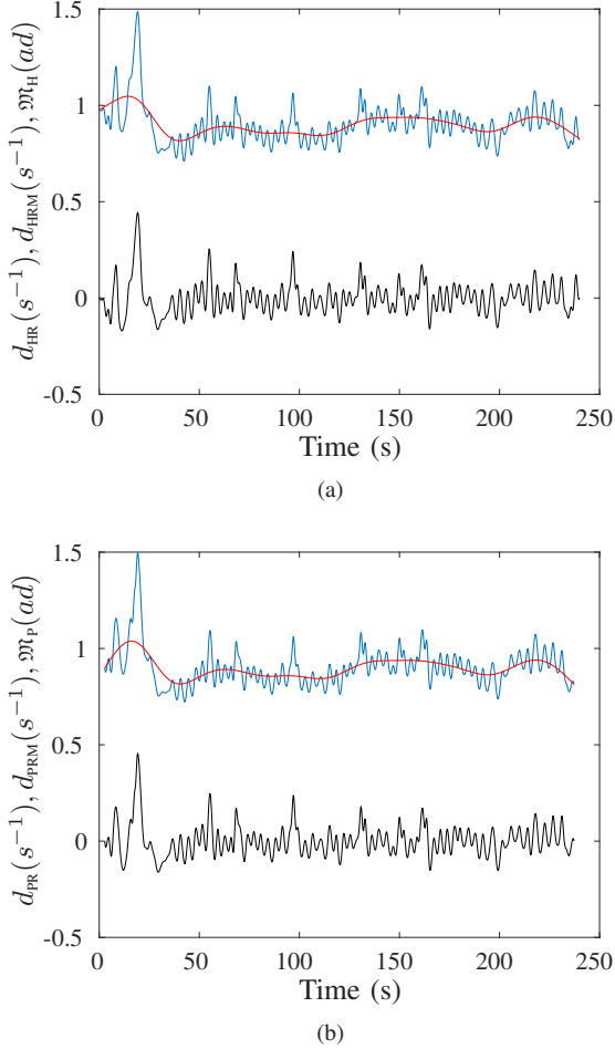
Fig. 2. d_{XR}(n) (in blue), d_{XRM}(n) (in red) and \mathfrak{M}_X(n) (in black) extracted from the ECG (a) and from the PPG (b).
