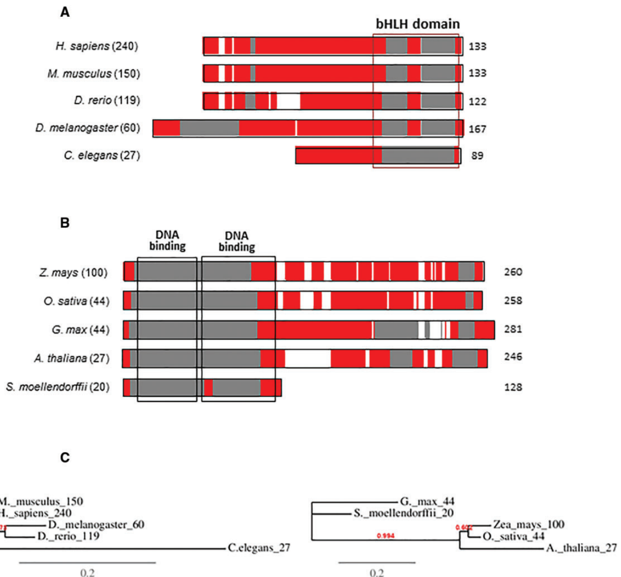
Fig. 5. —Comparison of orthologues from the bHLH and MYB TF families. Alignments of orthologue proteins encode by (A) NHLH1 gene from H. sapiens (Q02575), M. musculus (Q02576), D. rerio (Q6P0A8), D. melanogaster (O77278) and C. elegans (Q18590) and (B) MYB13 orthologues from Z. mays (K7TYD9), O. sativa (Q6K1S6), Glycine max (Q0PKJ2), A. thaliana (Q9LNC9) and S. moellendorffii (D8RNQ0). The number of cell types is given between parentheses on the left side of the sequence. The protein length is written on the right side of the sequence. Sequences are represented by color coded bars representing predicted disorder: disordered residues (red), ordered residues (grey), and alignment gaps (white). (C) Maximum likelihood trees of NHLH1 (left panel) and MYB13 (right panel) sequences used in the alignments. The specie name and the corresponding number of cell types are given in the tree.
