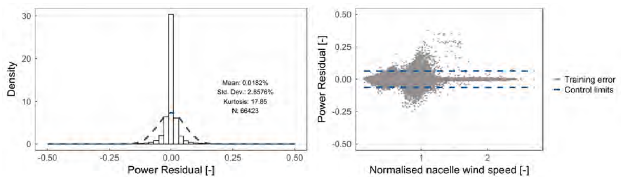
Figure 7. Training error statistics and distribution from RF model (left side); the related normal distribution is illustrated in blue. Training error (grey) and related control limits (blue) from RF model varying depending on the wind speed (right side).
