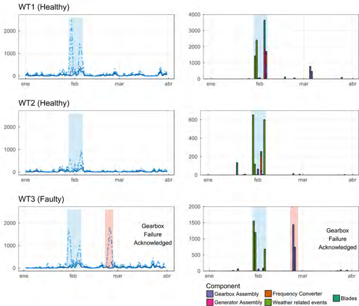
Figure 12. Detection of daily underperformance events (left) and corroborated component-related root cause (right). Alignment of the two are noted by their co-occurrence in the shaded regions; the blue shaded area corresponds to the storm event and the red shaded area corresponds to the underperformance detected in the faulty WT.
