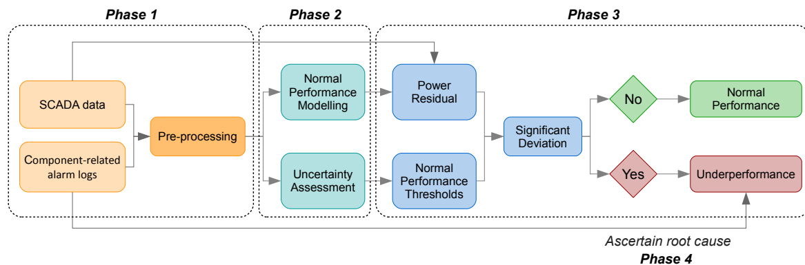
Figure 1. General framework for wind turbine performance monitoring.
