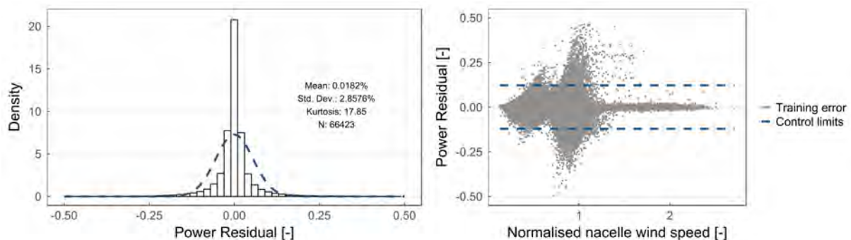
Figure 6. Training error statistics and distribution from kNN model (left side); the related normal distribution is illustrated in blue. Training error (grey) and related control limits (blue) from kNN model varying depending on the wind speed (right side).
