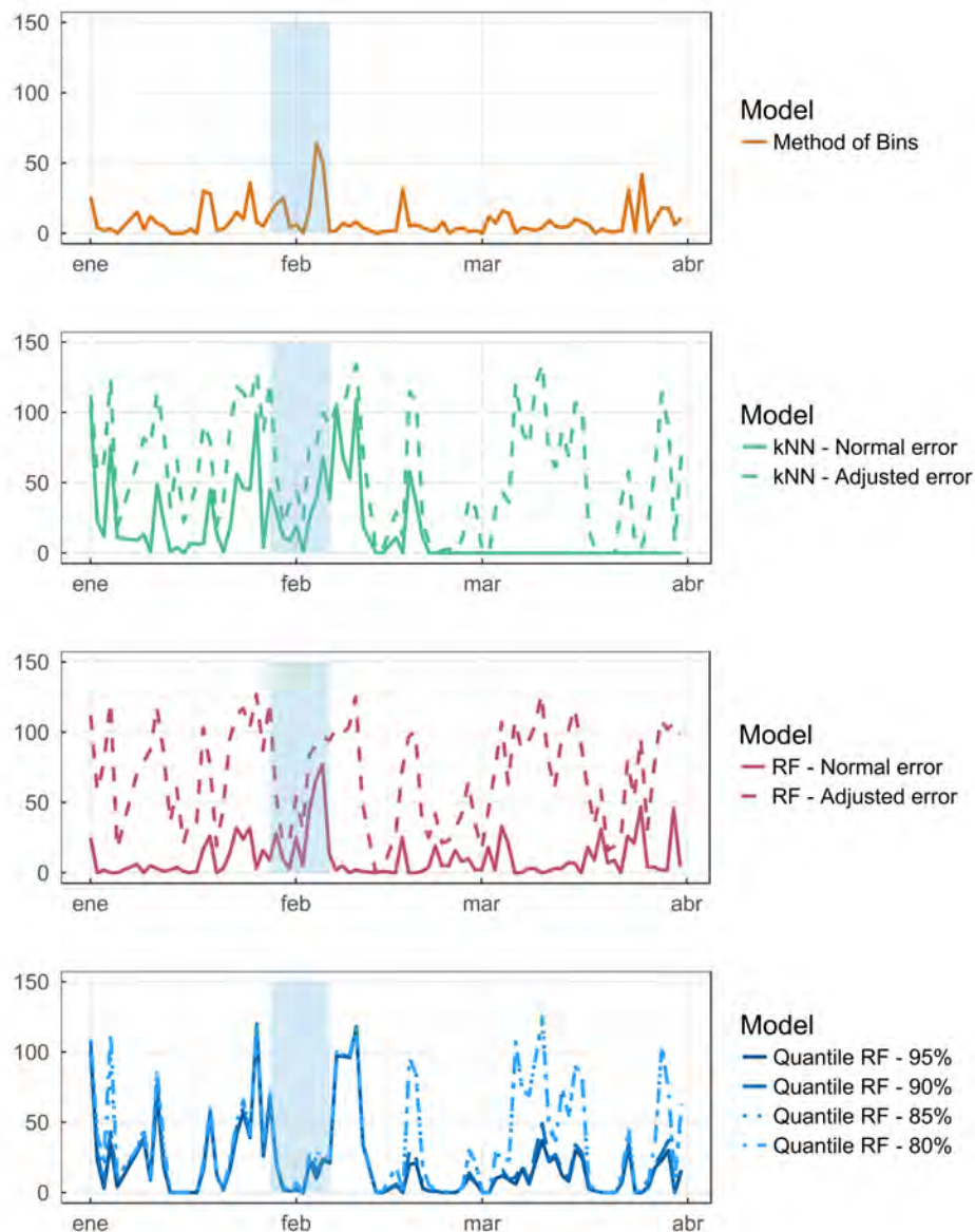
Figure 10. Daily monitoring of a healthy WT using 10-minute SCADA data: cumulative daily number of underperformance events detected with four different modelling approaches. The blue shaded area represents a storm event.
