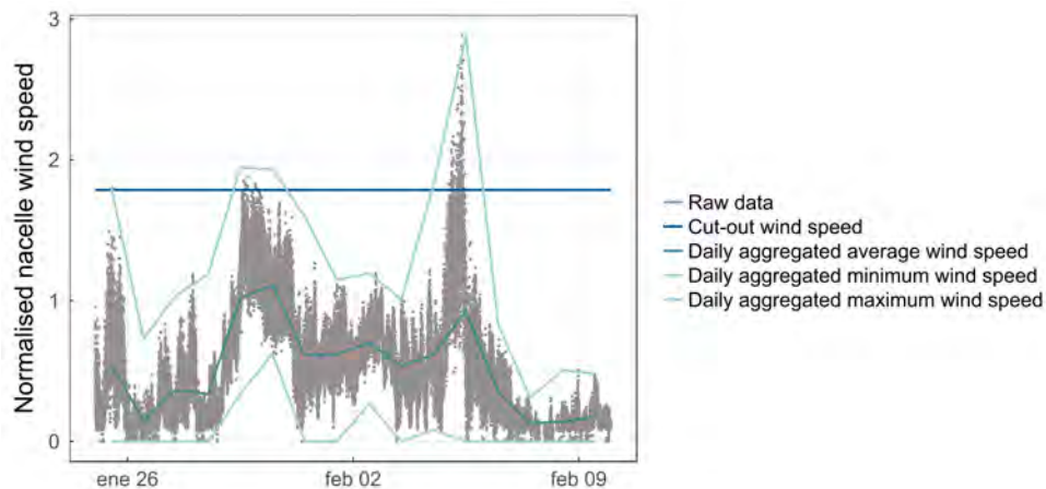
Figure 11. Nacelle wind speed data recorded during the storm event as reported in the alarm logs.
