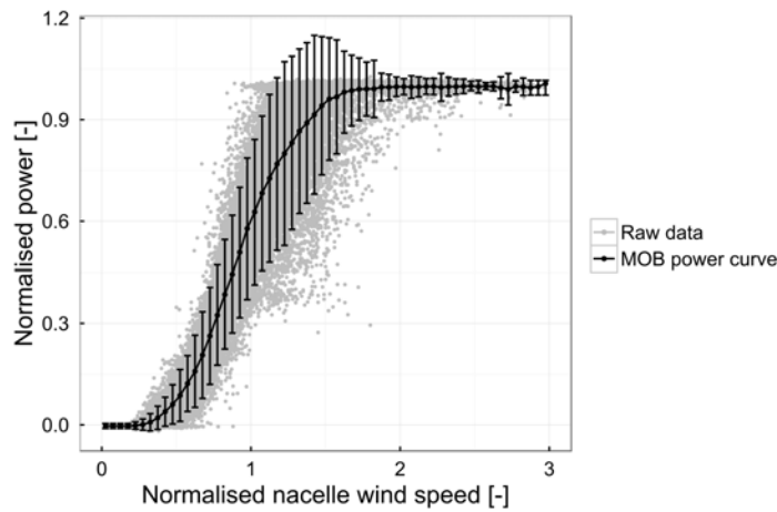
Figure 3. Power curve and related uncertainty derived from the MOB.
