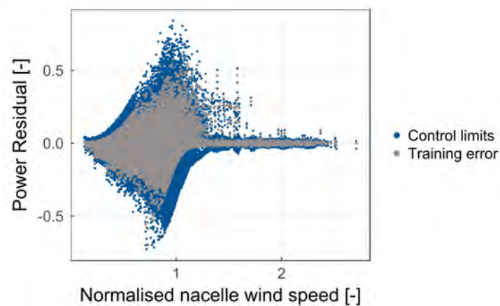
Figure 5. Training error (grey) and related control limits (blue) from the MOB varying depending on the wind speed.
