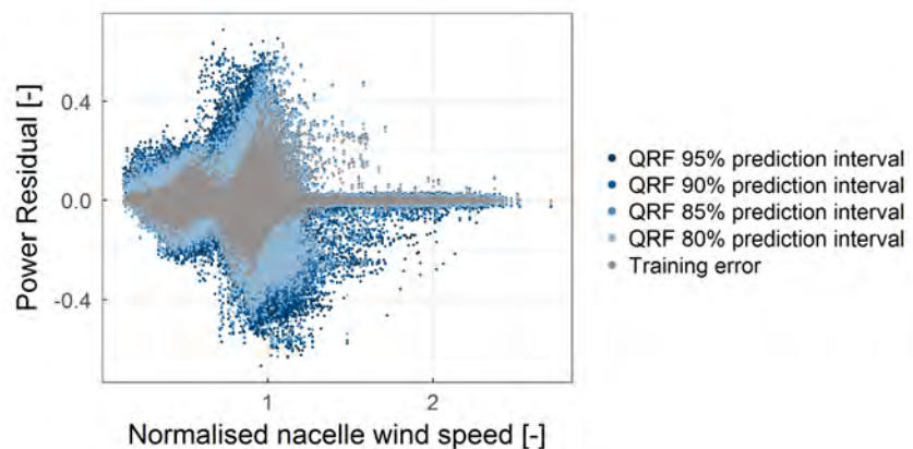
Figure 8. Training error (grey) and related control limits (4 shades of blue) from the QRF varying depending on the wind speed.
