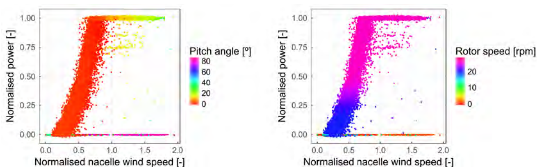
Figure 2. Scatter WT power curve varying depending on blade pitch angle (left) and rotor speed (right).
