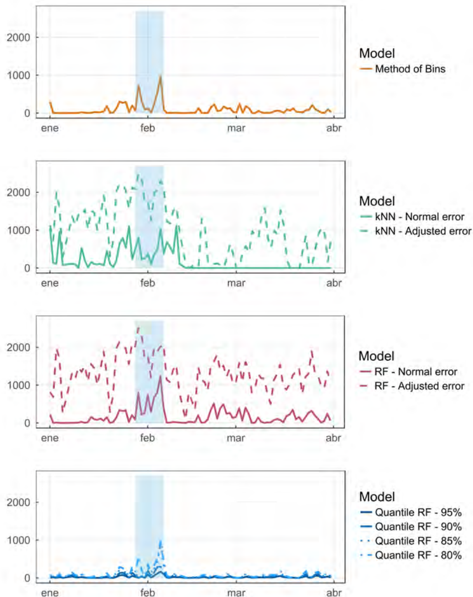
Figure 9. Daily monitoring of a healthy WT using high-frequency SCADA data: cumulative daily number of underperformance events detected with four different modelling approaches. The blue shaded area represents a storm event.
